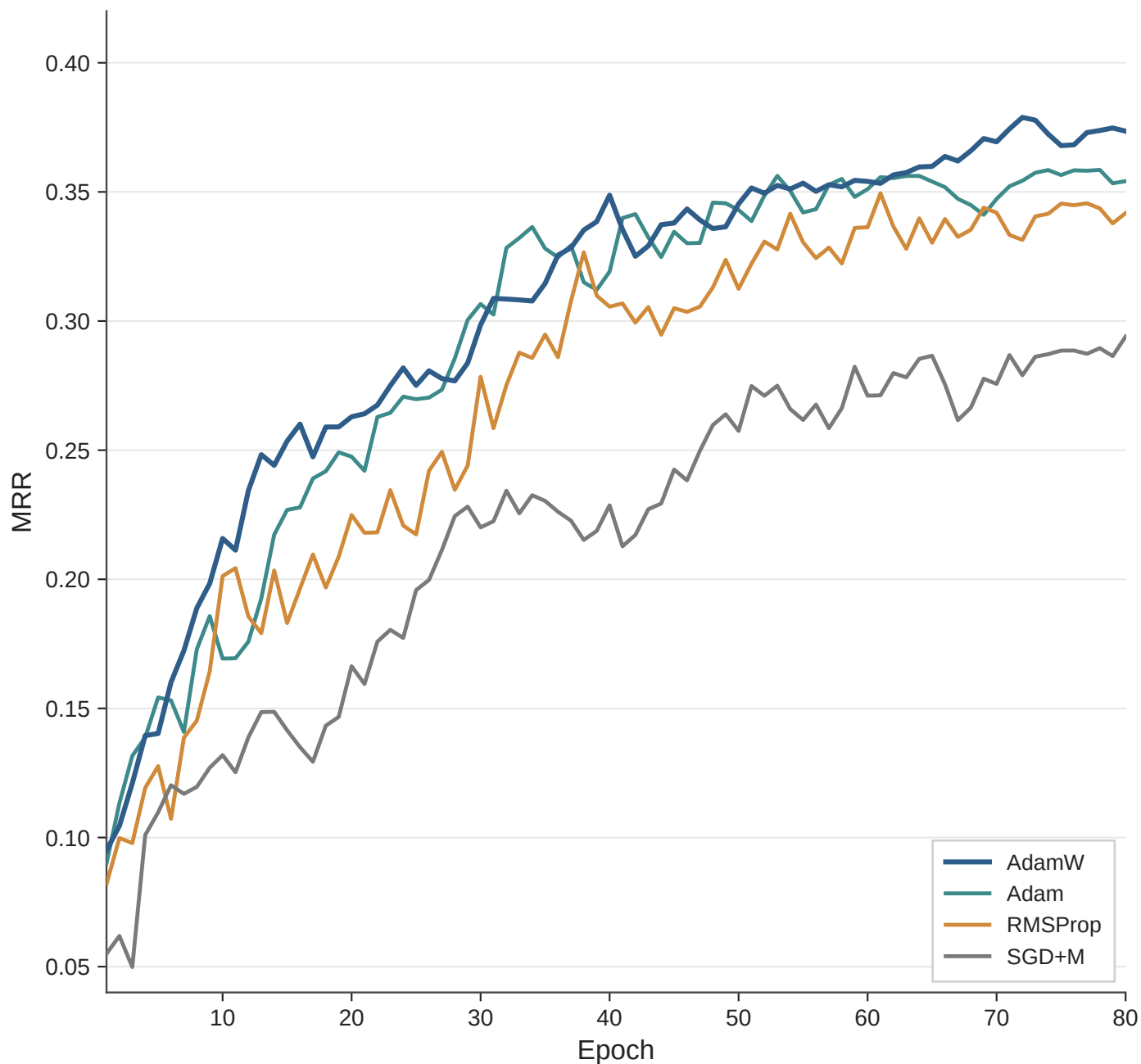
Optimizer Comparison on Validation MRR
