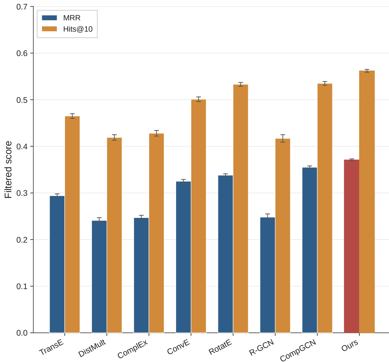
Knowledge Graph Embedding Comparison
