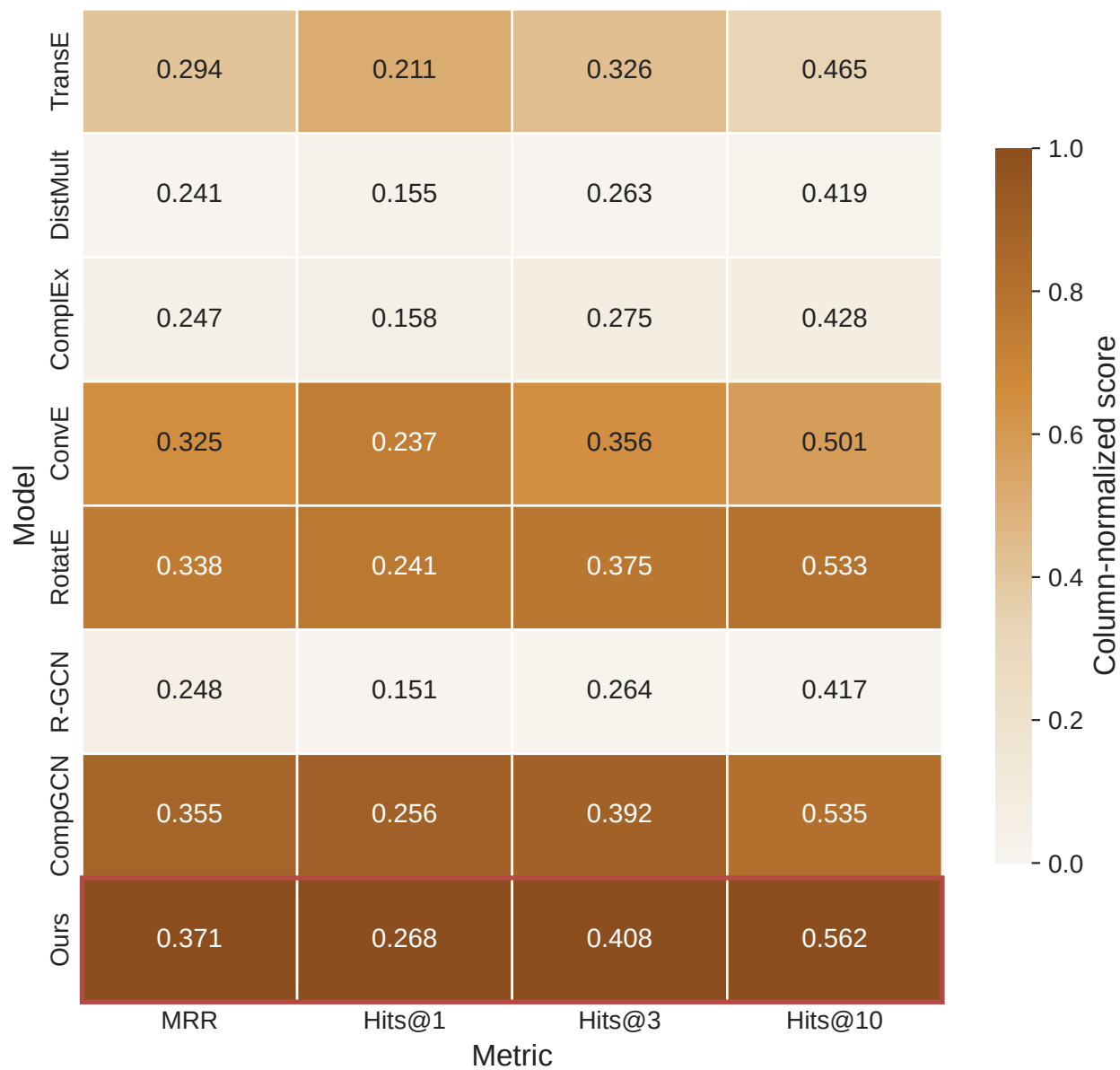
Final Link-Prediction Metrics
