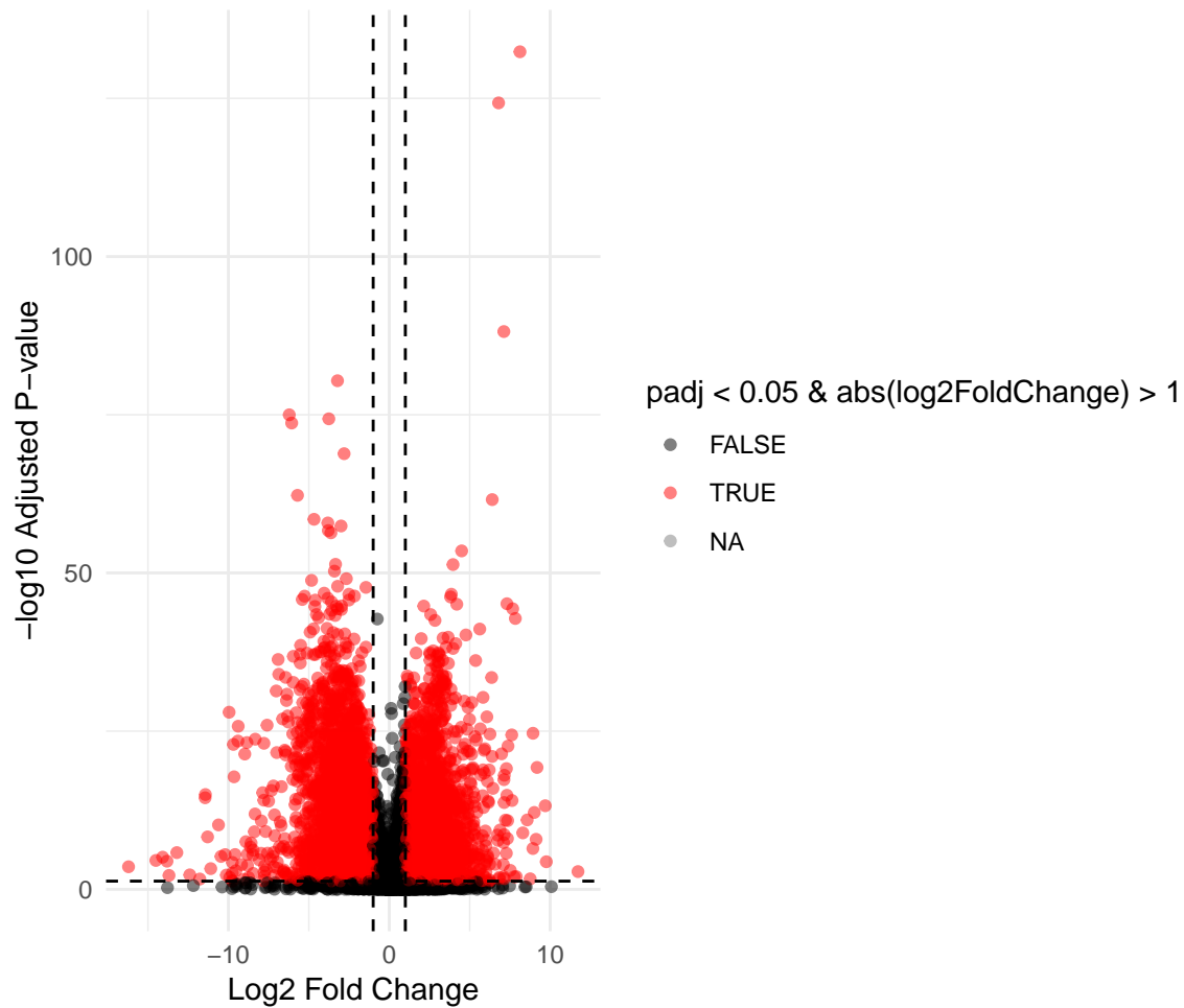
Volcano Plot (ggplot2)
