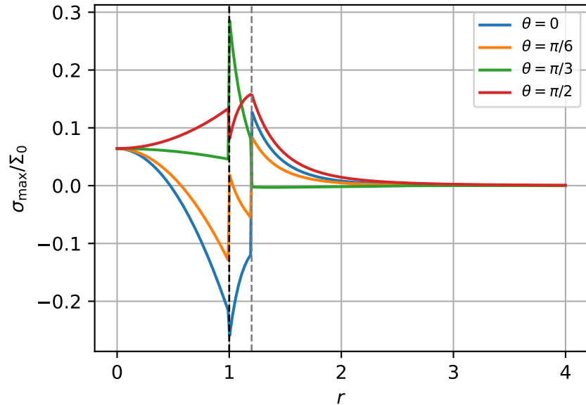
Maximum principal stress
