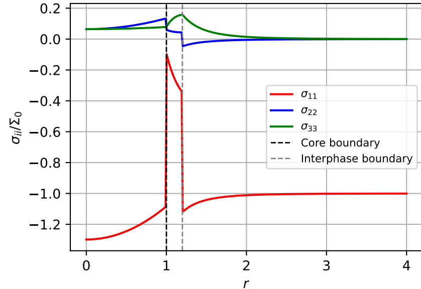
Stress components at \theta = \pi/2
