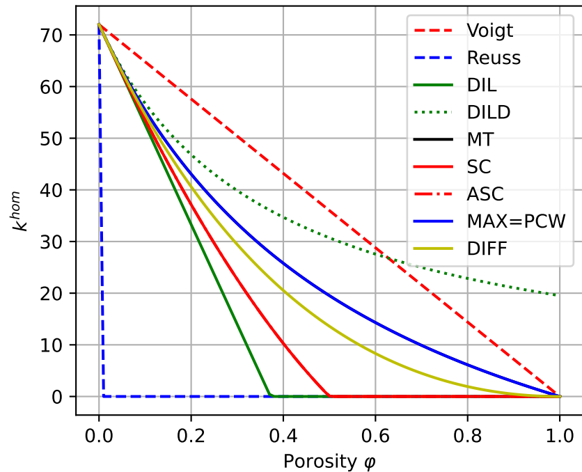
Bulk modulus
