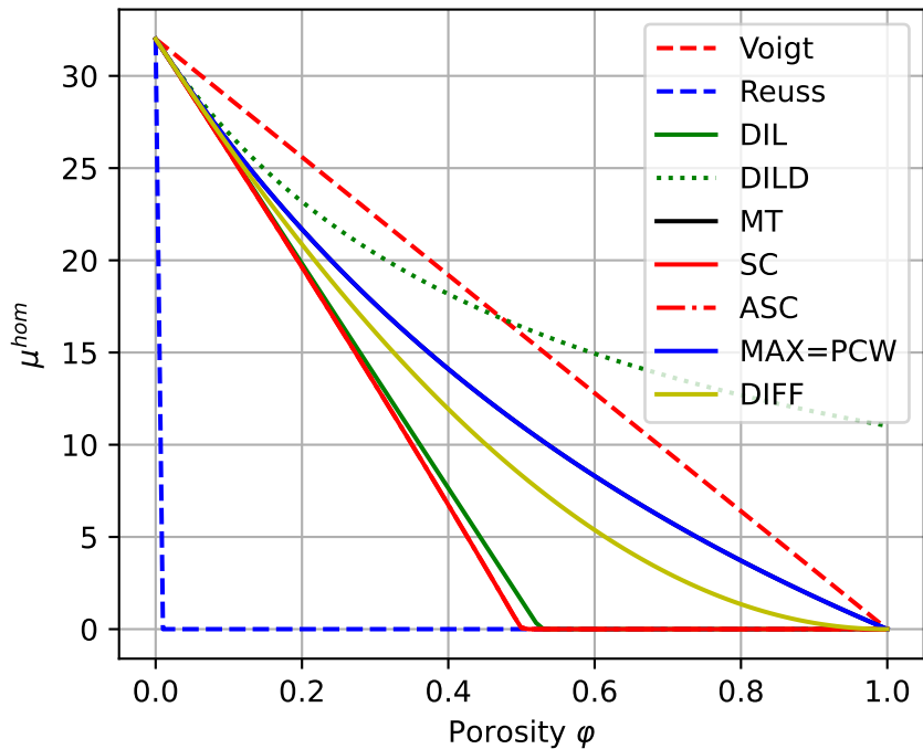
Shear modulus
