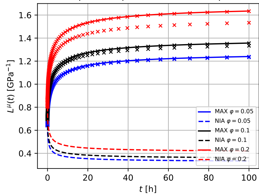
Spherical pores — shear creep
