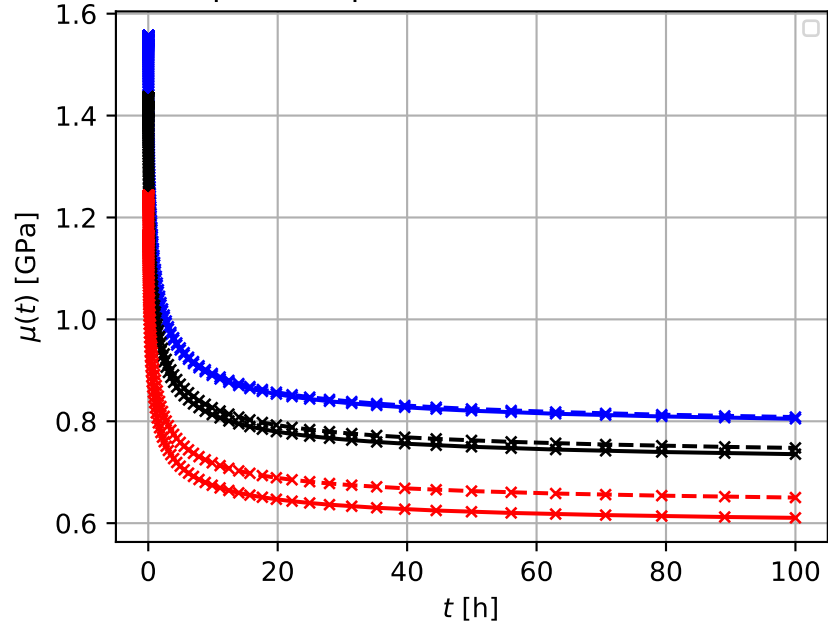
Spherical pores — shear relaxation
