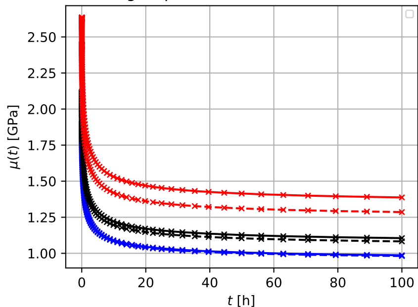
Spherical pores — shear relaxation
