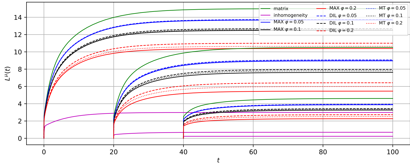
Shear creep — effect of scheme and volume fraction, \omega = 0.1
