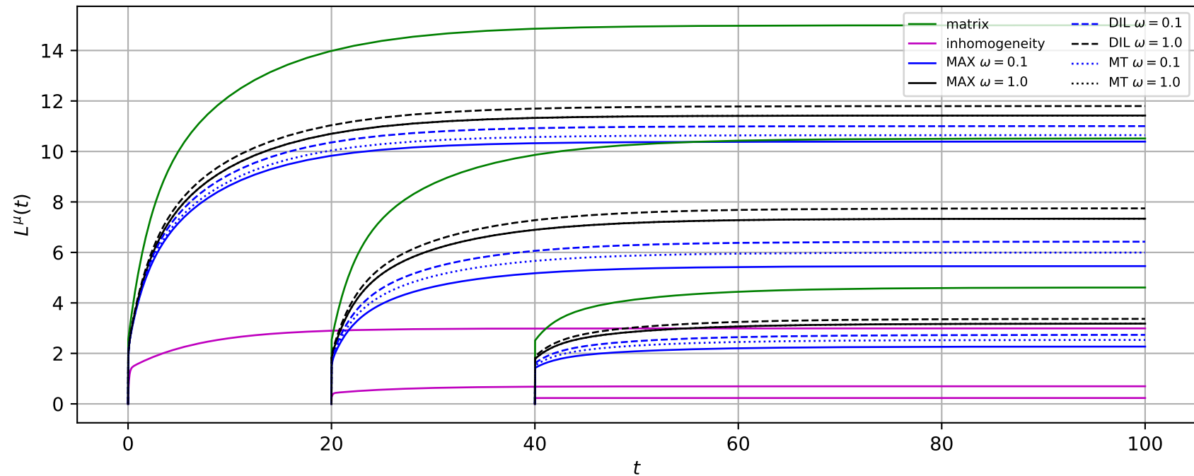
Shear creep — effect of scheme and aspect ratio, \phi = 0.2
