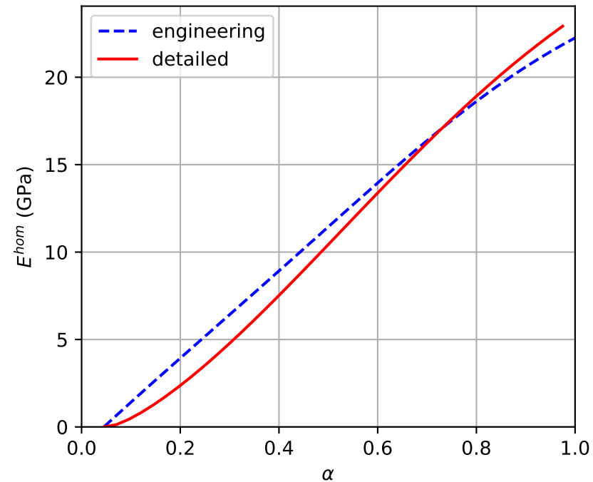
Young's modulus — w/c=0.4
