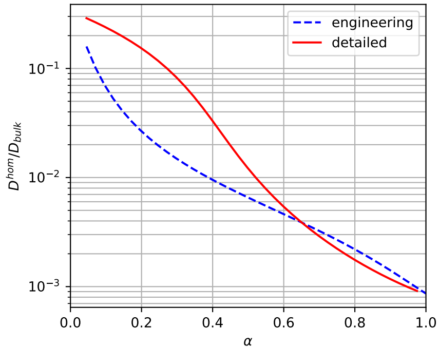
Chloride diffusivity — w/c=0.4
