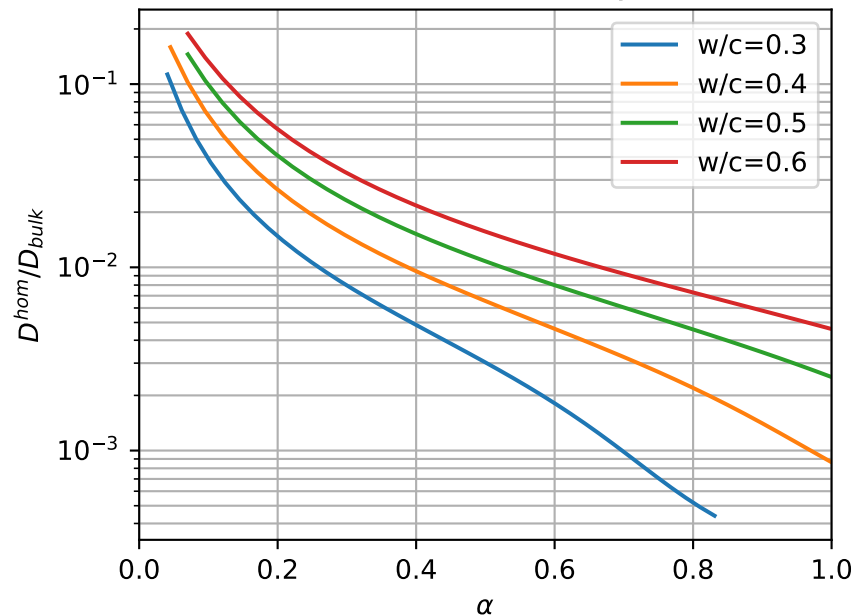
Chloride diffusivity
