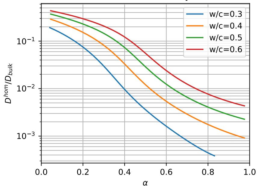
Chloride diffusivity
