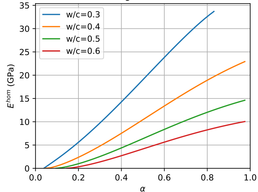
Young's modulus
