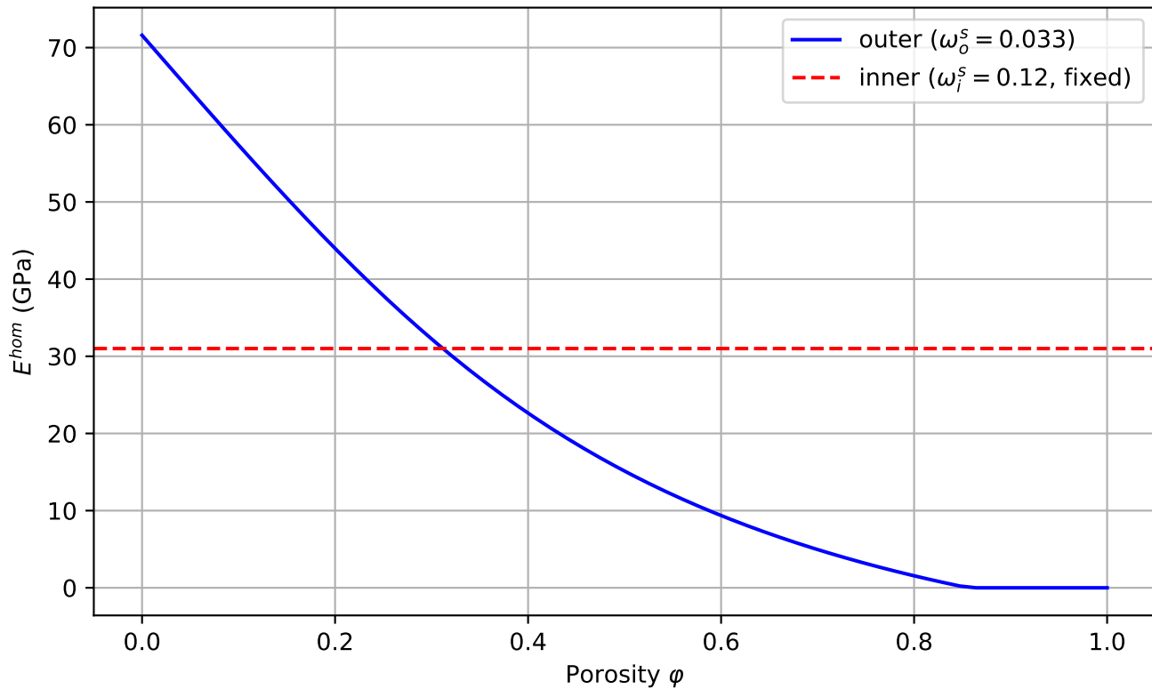
SC estimates of inner and outer C-S-H
