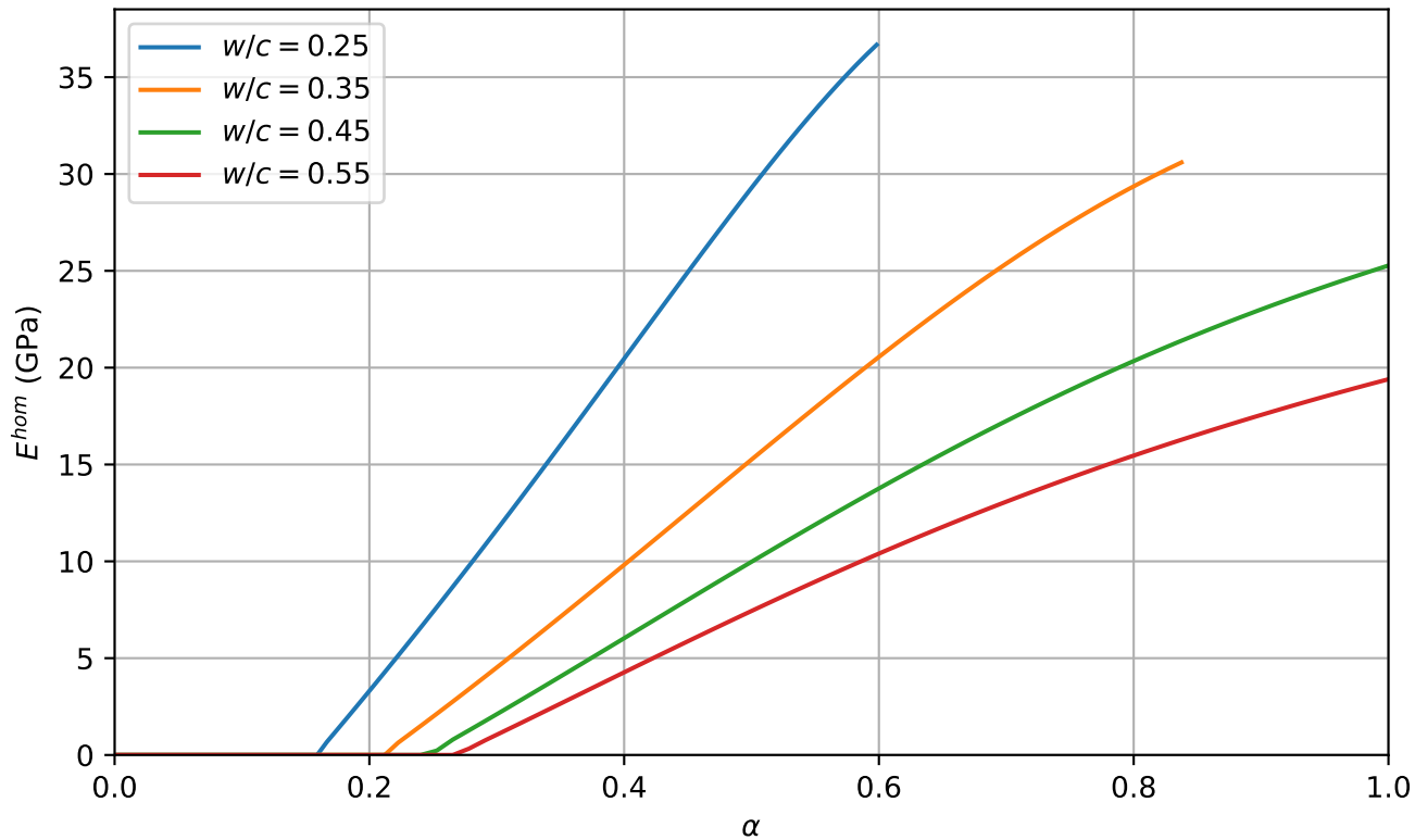
Drained Young's modulus of cement paste
