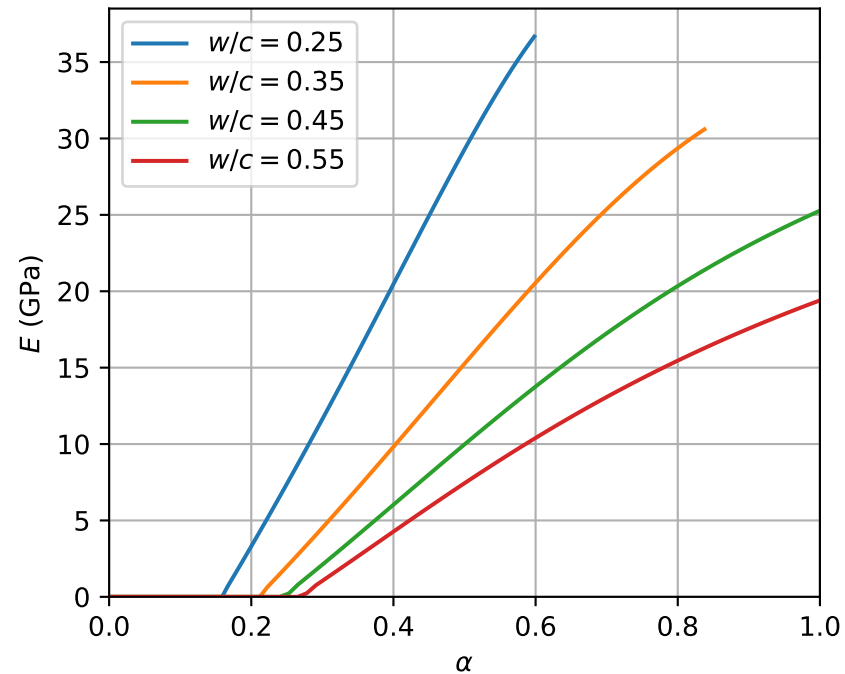
Drained E^{hom}
