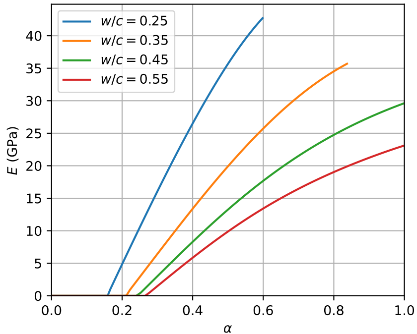
Undrained E^{hom,u}
