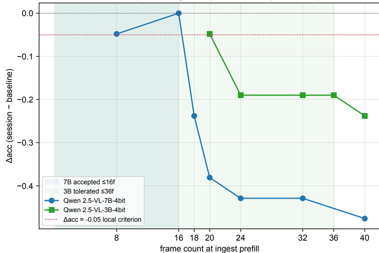
Follow-up accuracy cost (tested envelope shaded)
