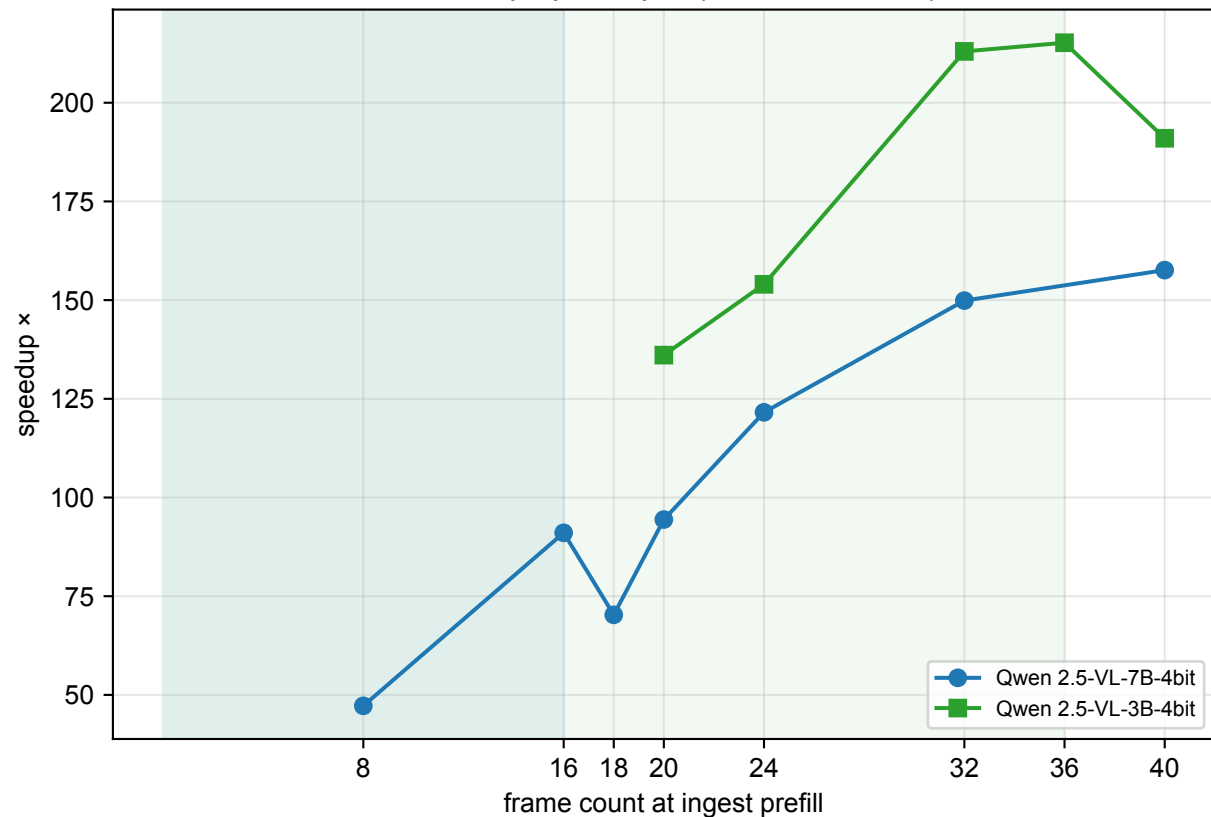
Follow-up speedup \times (dense / session)
