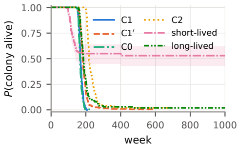
(a) survival of colonies
