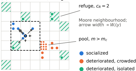
(a) lattice, motion, refuges
