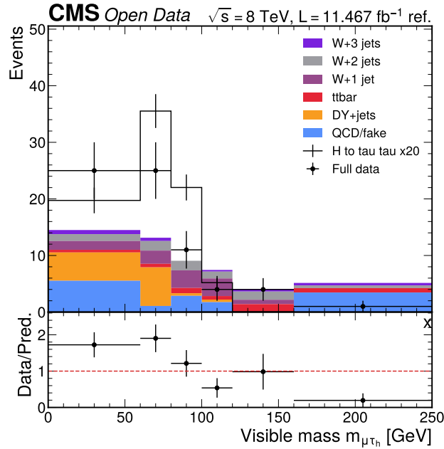
Figure 14: Visible-mass baseline in the VBF category. The plot compares data with the baseline visible-mass prediction after the data-driven reducible-background correction. The lower panel shows the data-to-prediction ratio.
