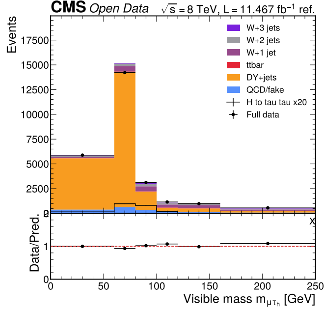
Figure 16: Visible-mass baseline in the zero-jet category. The plot compares data with the baseline visible-mass prediction in the statistically dominant category. This category controls the global normalization behavior of the baseline workspace.
