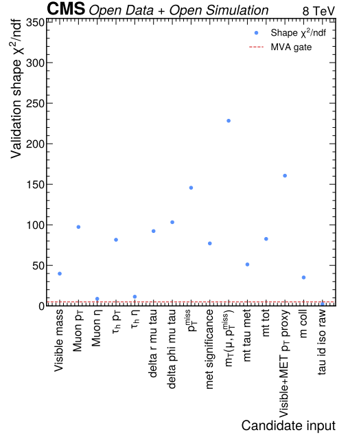
Figure 10: MVA input modelling summary. The figure records the data/background modelling quality of candidate classifier inputs. It documents the validation context for using a single retained D_{NN} tool.
