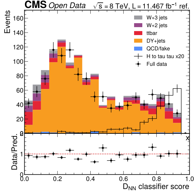
Figure 18: D_{NN} score in the boosted category. The plot compares data with the retained classifier-score prediction in the boosted category. The ratio panel checks whether the classifier ordering is modelled in observed data.
