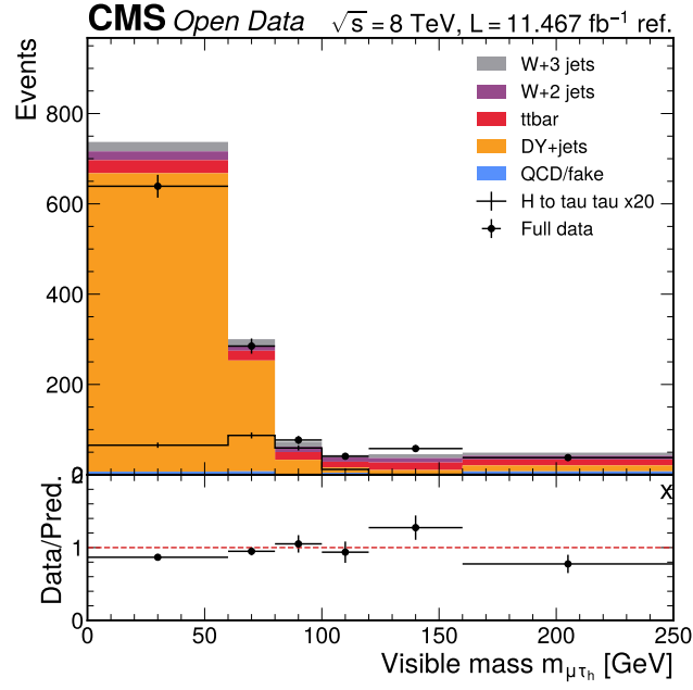
Figure 15: Visible-mass baseline in the boosted category. The plot compares data with the baseline visible-mass prediction in the boosted category. This category has substantially more events than the VBF category and constrains the broad visible-mass shape.
