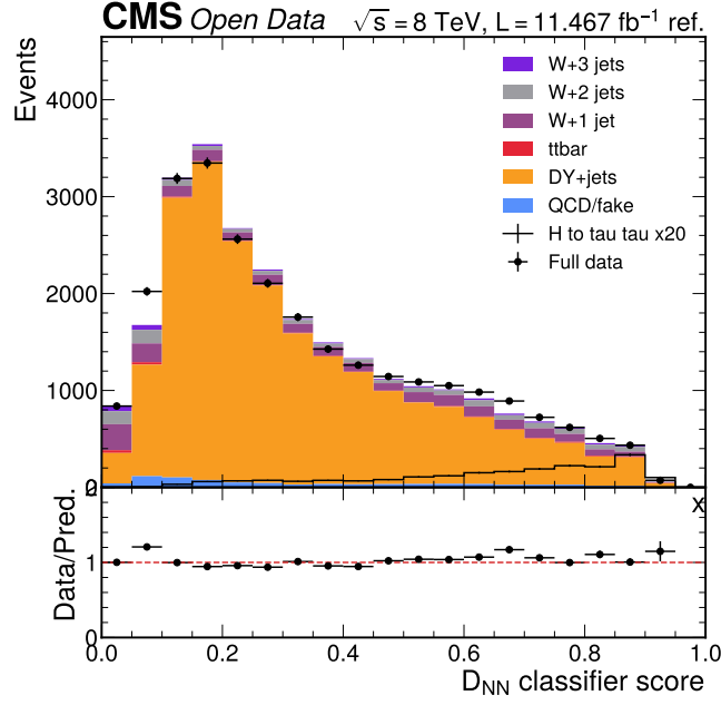
Figure 19: D_{NN} score in the zero-jet category. The plot compares data with the retained classifier-score prediction in the zero-jet category. The category has the largest statistical weight in the combined classifier fit.
