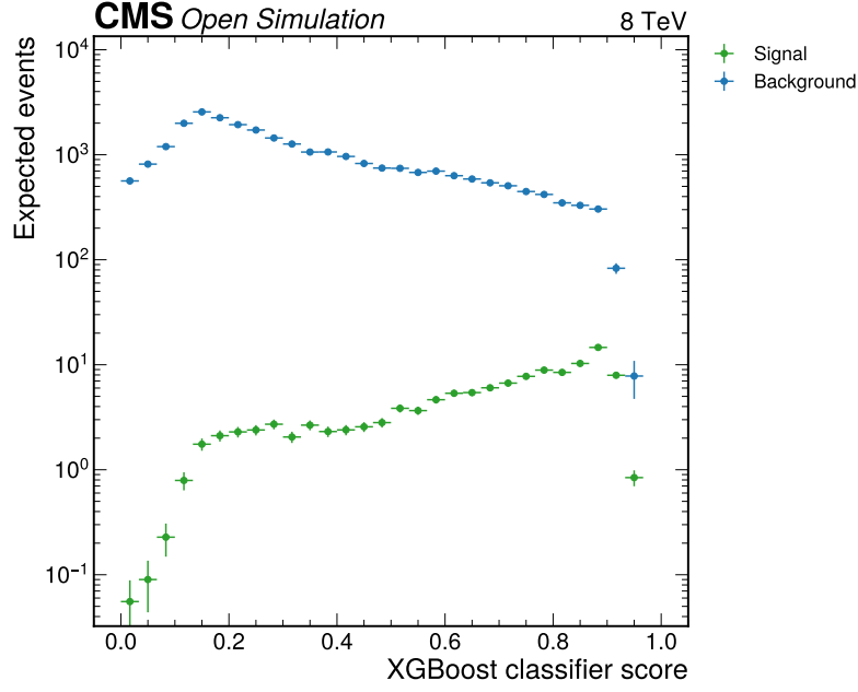
Figure 11: Expected classifier score templates. The figure shows the trained classifier score response for signal and background before observed-data fitting. It checks that the retained classifier has the intended signal/background ordering.
