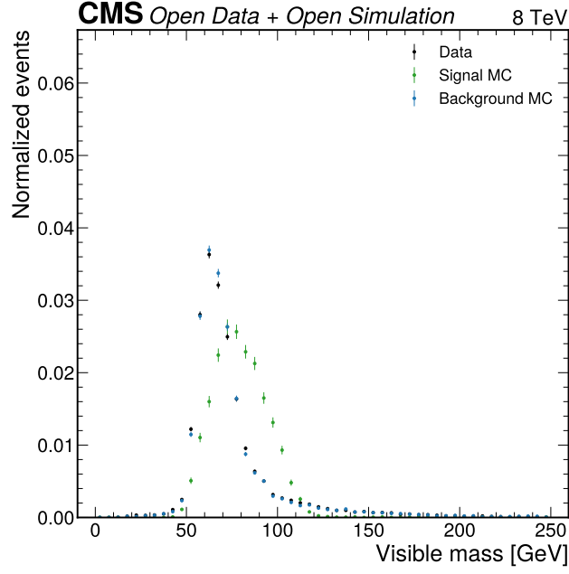
Figure 9: Visible-mass distribution in the zero-jet category. The pre-fit comparison shows the broad baseline observable in the highest-statistics category. It anchors the background-rich part of the simultaneous fit.
