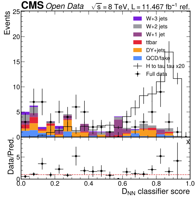
Figure 17: D_{NN} score in the VBF category. The plot compares data with the retained classifier-score prediction in the VBF category. The same score definition and binning are used in the other categories.
