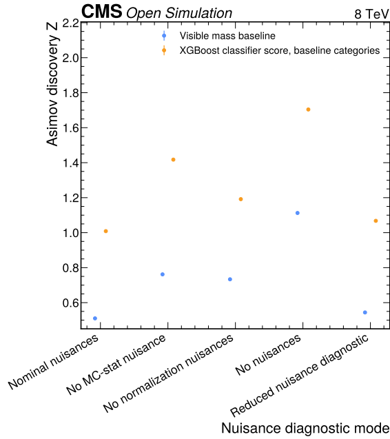
Figure 13: Sensitivity nuisance audit. The figure summarizes the expected sensitivity response to the retained nuisance model. It is used to confirm that the current results are not driven by a hidden no-systematics configuration.
