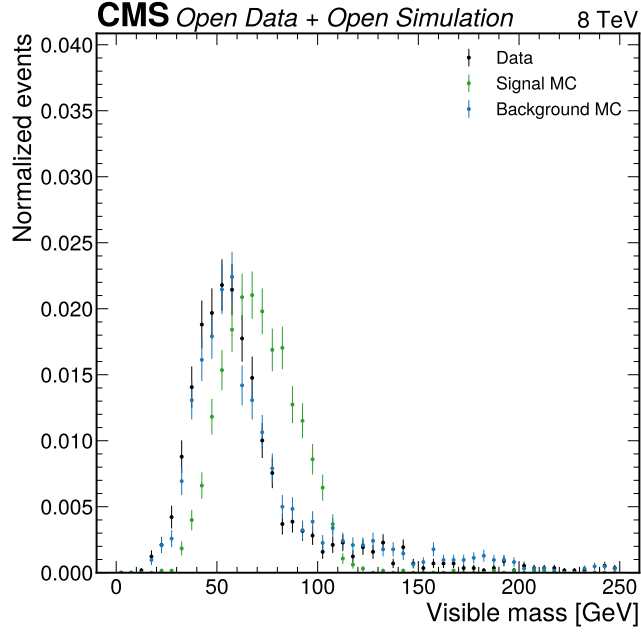
Figure 8: Visible-mass distribution in the boosted category. The pre-fit comparison shows the baseline observable in the recoil-enhanced category. This is a major contributor to the simultaneous visible-mass baseline fit.
