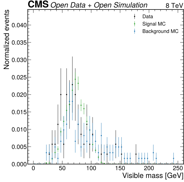
Figure 7: Visible-mass distribution in the VBF category. The pre-fit comparison shows the fitted baseline observable in the most signal-enriched topology. The final fit uses the corresponding Phase-4c template with the same category definition.
