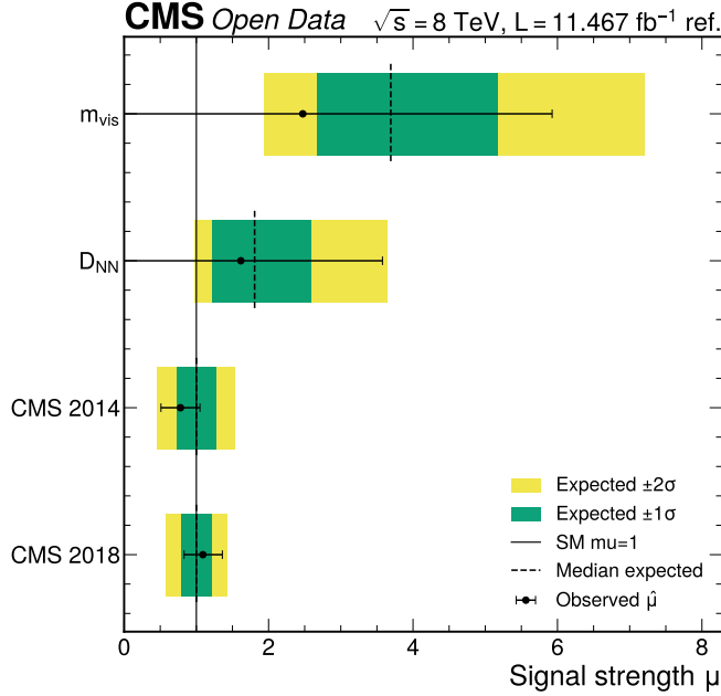
Figure 20: Observed result summary. The figure compares the visible-mass baseline, retained D_{NN} result, CMS 2014 result, and CMS 2018 result on the same signal-strength scale. Each row uses the same convention: black observed point with horizontal uncertainty, green and yellow expected one- and two-standard deviation bands, a black dashed median-expected marker, and the common Standard Model line at \mu = 1 .
