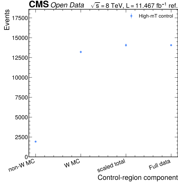
Figure 12: W high- m_T control-region scale. The figure shows the non- W MC, nominal W MC, scaled control-region prediction, and observed data in the high- m_T control region. This scale is propagated to both retained workspaces.
