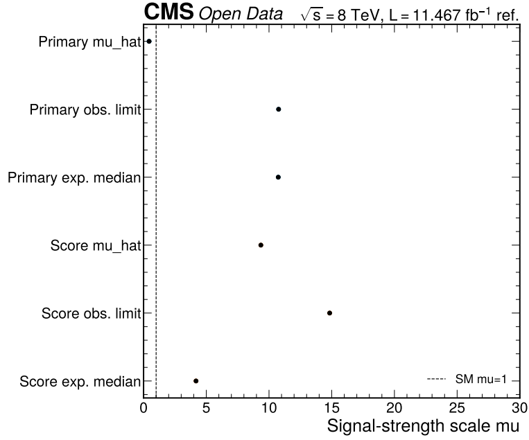
Figure 7: Observed limit and significance summary. The figure shows the primary visible-mass fit and the score-template diagnostic on the same signal-strength scale. The score result is flagged and not CMS-quality evidence.
