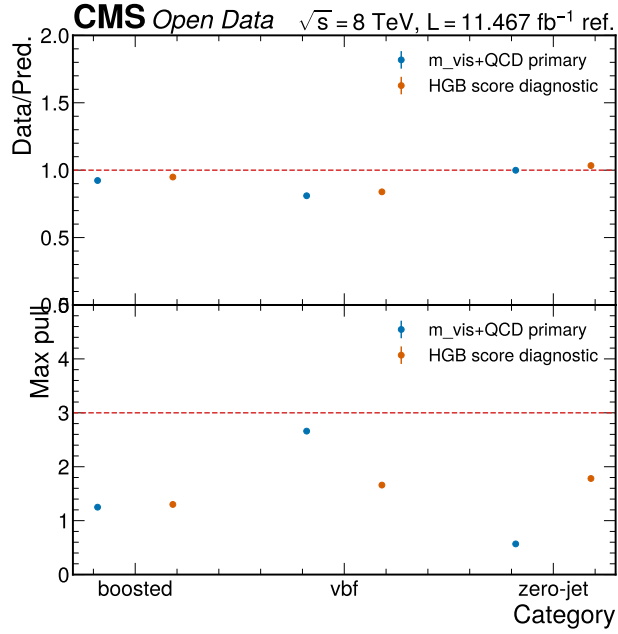
Figure 6: Observed pull and ratio summary. The figure compares primary visible-mass and score-template validation behavior after the QCD/fake audit correction. It is the central diagnostic for why the visible-mass result is primary and the score fit is diagnostic only.
