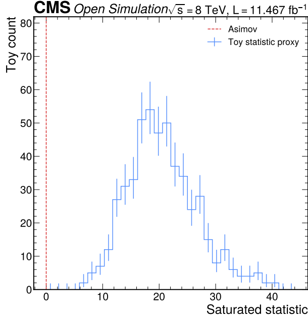
Figure 16: Limited toy GoF distribution. The toy distribution is generated from background-only expected templates and compared with the Asimov saturated statistic. The vertical marker at zero is expected by construction, so the figure validates toy generation and statistic evaluation rather than real-data agreement.
