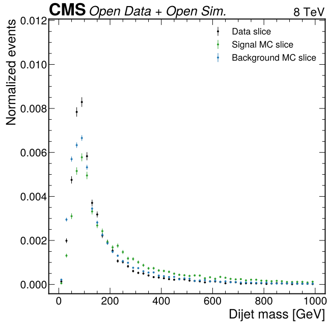
Figure 28: Phase 2 dijet mass diagnostic. The first-candidate survey showed that leading-dijet mass is available and populated enough to study a VBF-like category. The final VBF diagnostic is shown in Figure 12.
