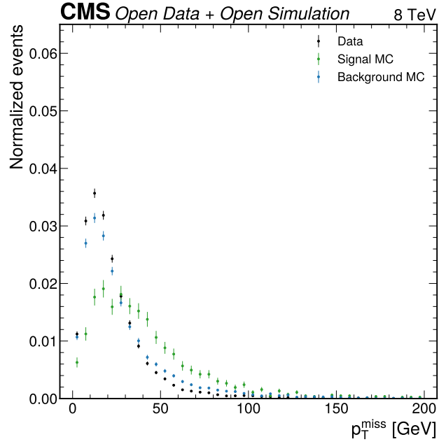
Figure 8: Missing transverse momentum. The Phase 3 MET comparison documents the reconstructed missing-momentum input used for transverse mass and add-MET diagnostics. It also illustrates why MET-sensitive alternative observables remain cross-checks rather than promoted primary fit variables in this reduced model.
