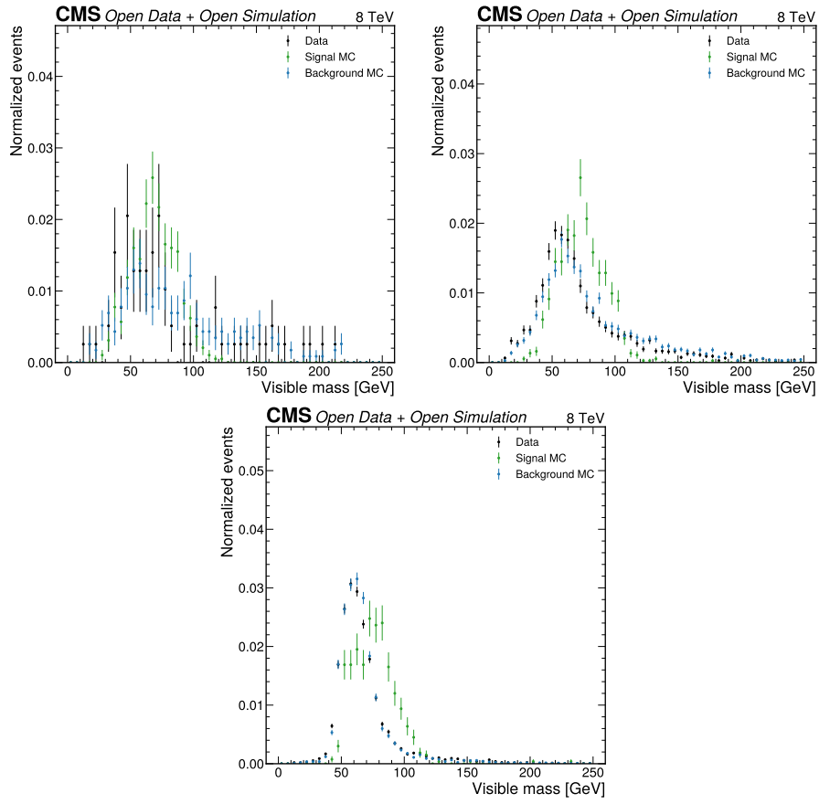
Figure 31: Phase 3 visible-mass diagnostics by category. From left to right, the panels show the VBF, boosted, and zero-jet categories before the Phase 4a expected model added official Open Data normalization. The Phase 4a expected templates in Figures 19, 19, and 19 supersede these normalized diagnostics for the expected statistical model.
