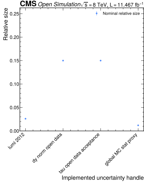
Figure 14: Expected nuisance summary. This Phase 4a diagnostic ranks implemented rate and MC-stat uncertainty handles in the expected workspace. It is not an observed-data post-fit impact plot; it shows the nuisance structure available before 10% validation and full unblinding.
