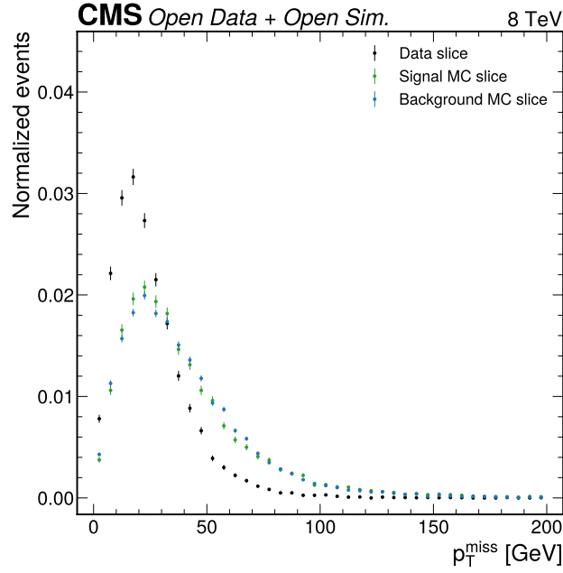
Figure 23: Phase 2 MET diagnostic. This plot established that reconstructed MET is available in the reduced files and can support transverse-mass and add-MET studies. It also helped identify the absence of direct GenMET needed for the requested NN genMET regression.
