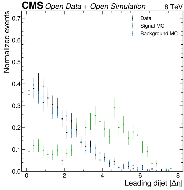
Figure 13: Leading dijet pseudorapidity separation. This selected-event distribution supports the VBF category requirement on the leading-dijet absolute eta separation. It also passed the Phase 3 MVA input-quality gate, but the classifier path was still downscoped because most other inputs failed.
