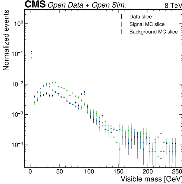
Figure 24: Phase 2 visible-mass diagnostic. This first-candidate visible-mass plot showed that m_{vis} can be constructed but also warned about loose candidate-cleaning artifacts. Phase 3 rebuilt the mass templates after final object selection before Phase 4a used them.
