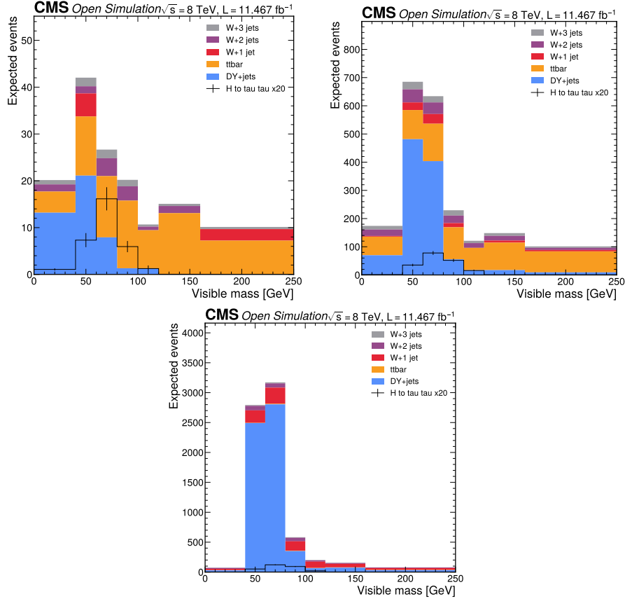
Figure 19: Expected visible-mass templates by fit category. From left to right, the panels show the VBF, boosted, and zero-jet categories with background-only expected stacks and nominal Higgs signal overlays after official Open Data normalization. The fit observation is the Asimov background expectation, not real collision data.
