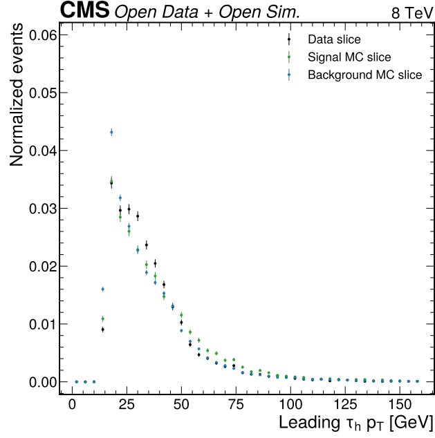
Figure 22: Phase 2 leading tau transverse momentum. This first-candidate plot confirmed that the tau candidate branches are populated in data and MC. The final \tau_h selection used for templates is documented by Figure 7.
