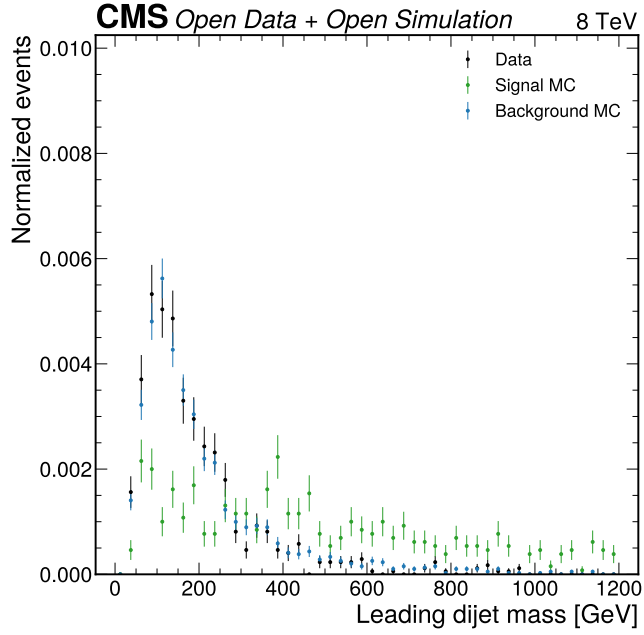
Figure 12: Leading dijet mass. The selected dijet-mass distribution supports the VBF-enriched category definition and was one of the few candidate MVA inputs to pass the Phase 3 modelling gate. The category threshold at 300 GeV is therefore retained as a transparent VBF-like requirement.
