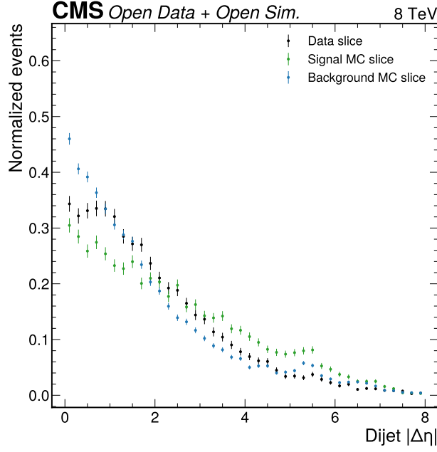
Figure 29: Phase 2 dijet eta-separation diagnostic. This plot identified leading-dijet eta separation as one of the strongest simple discriminators in the early survey. The final selected distribution in Figure 13 supports the retained VBF category.
