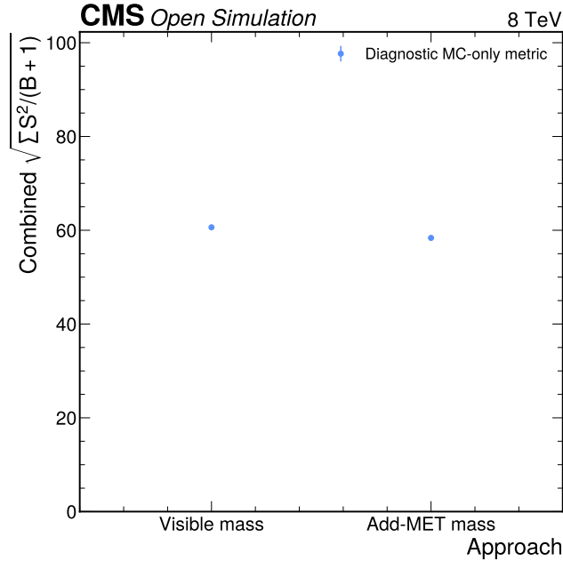
Figure 17: Approach comparison. The Phase 3 plot compares visible mass and add-MET mass using the same raw MC-only binned separation metric across the exclusive categories. Visible mass remains the Phase 4a primary because it has the better diagnostic metric and because add-MET has not passed a full nuisance-constrained expected-sensitivity replacement gate.
