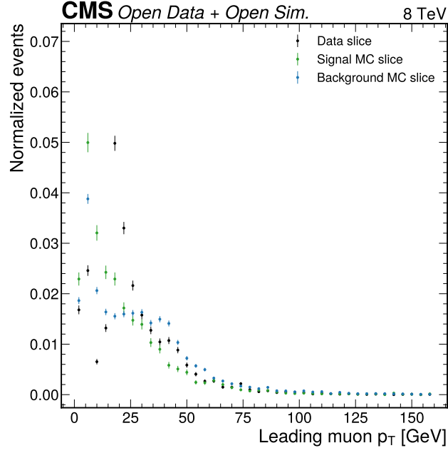
Figure 21: Phase 2 leading muon transverse momentum. This first-candidate slice check validated the presence and range of the muon branches before final object arbitration. It is included as provenance, while the final selected muon distribution in Figure 6 is the analysis-level diagnostic.
