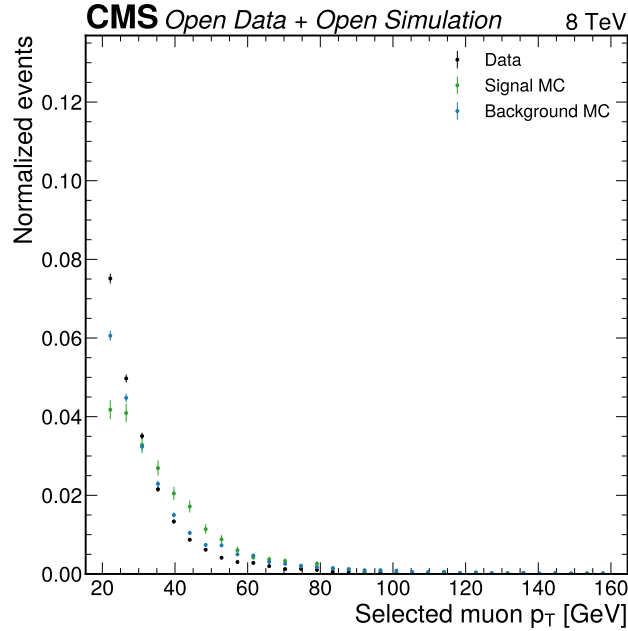
Figure 6: Selected muon transverse momentum. The Phase 3 plot uses final selected muons after trigger, ID, isolation, object arbitration, and signal-region requirements. It documents the muon kinematic phase space entering the Phase 4a templates rather than the looser first-candidate survey from Phase 2.
