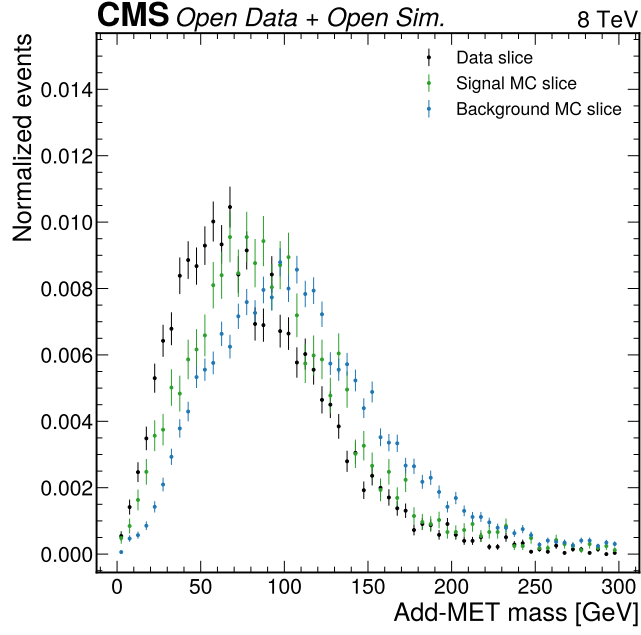
Figure 25: Phase 2 add-MET mass diagnostic. This plot demonstrated that a reconstructed-MET-assisted mass-like observable is available in both data and MC. The observable remains a documented alternative, but it is not the Phase 4a primary fit observable.
