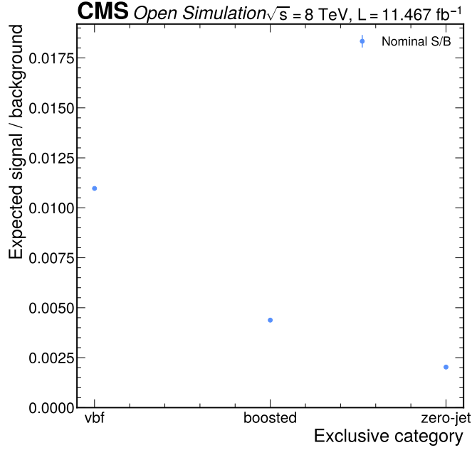
Figure 20: Expected signal-to-background ratio. This figure summarizes the category-integrated nominal Higgs signal divided by nominal background. The boosted category has the largest S/\sqrt{B} , while the VBF category remains important for topology coverage despite the small absolute signal yield.
