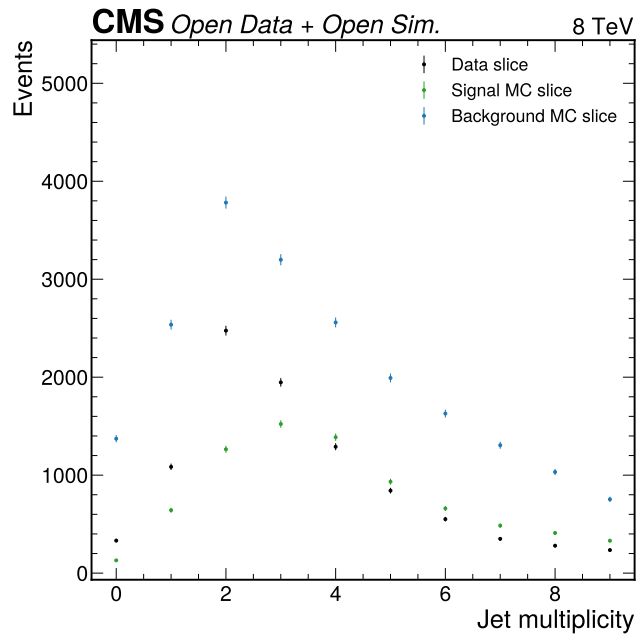
Figure 27: Phase 2 jet multiplicity diagnostic. This plot supported the feasibility of category construction with zero-jet, boosted, and VBF-like topologies. Final clean-jet multiplicity is documented by Figure 11.
