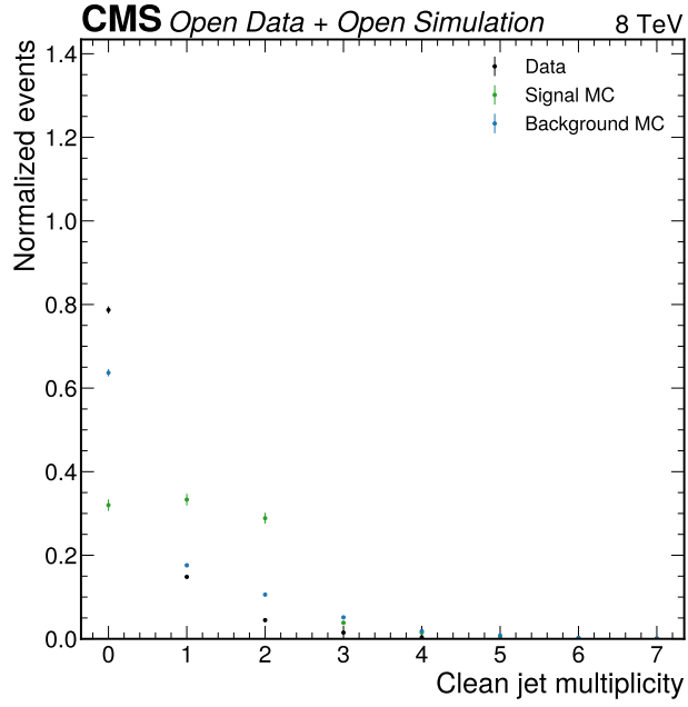
Figure 11: Clean jet multiplicity. The figure motivates the three retained fit categories by showing the selected-event jet multiplicity. The visible data/MC shape difference is one reason the analysis uses transparent category boundaries and avoids a trained classifier in Phase 4a.
