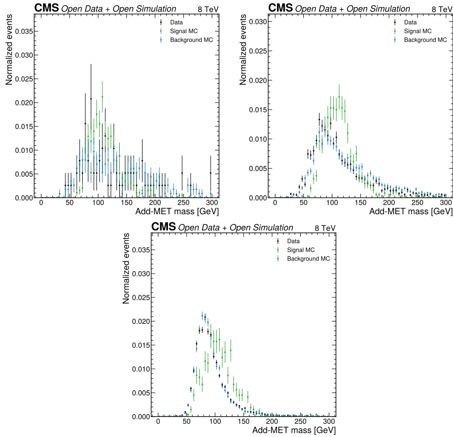
Figure 32: Phase 3 add-MET mass diagnostics by category. From left to right, the panels show the VBF, boosted, and zero-jet categories for the alternative observable retained for audit because add-MET mass was required by the user prompt. The observable supports the documented alternative-observable study but is not promoted over visible mass in Phase 4a.
