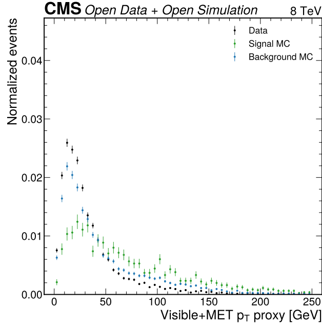
Figure 10: Visible-plus-MET transverse momentum proxy. This Phase 3 diagnostic records the available proxy for the boosted topology. The raw data/MC modelling was not sufficient for MVA promotion, but the variable remains part of the category and alternative-observable context.
