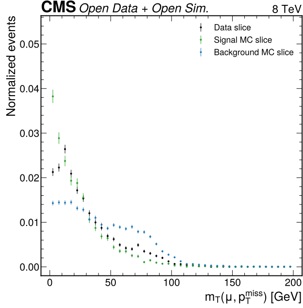
Figure 26: Phase 2 transverse-mass diagnostic. This first-candidate distribution motivated the low- m_T signal-region and high- m_T W control-region definitions. The final selected transverse-mass behavior is shown in Figure 9.
