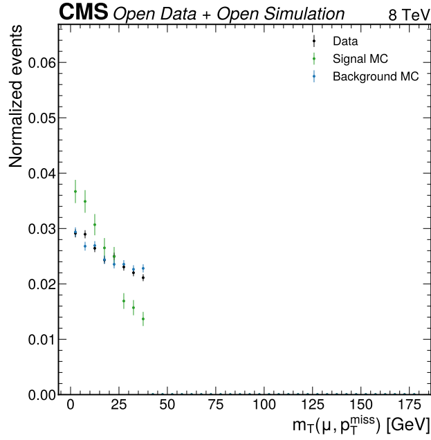
Figure 9: Muon-MET transverse mass. This distribution is shown after the low- m_T signal-region requirement and documents the variable that separates the signal-region candidate set from the high- m_T W control handle. The same quantity is deliberately not used as an MVA discriminant after Phase 3 validation failures in the broader input set.
