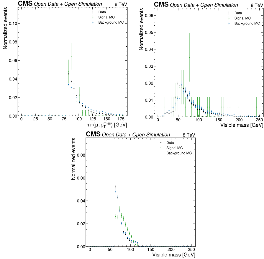
Figure 5: Phase 3 control and validation diagnostics. From left to right, the panels show the W high- m_T control-region shape comparison, the same-sign QCD sideband visible-mass comparison, and the Z-rich validation visible-mass comparison. These diagnostics document the available W+jets, fake-tau, and DY/Z handles while the Phase 4a expected model retains the corresponding limitations and does not tune these components to real data.
