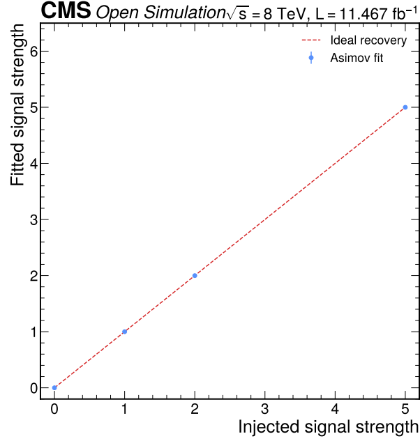
Figure 15: Signal-injection recovery. The Phase 4a injection study fits Asimov pseudo-data generated at injected signal strengths 0, 1, 2, and 5. The recovered signal strengths lie on the diagonal within the predeclared tolerance, which validates the workspace response under nominal model assumptions.
