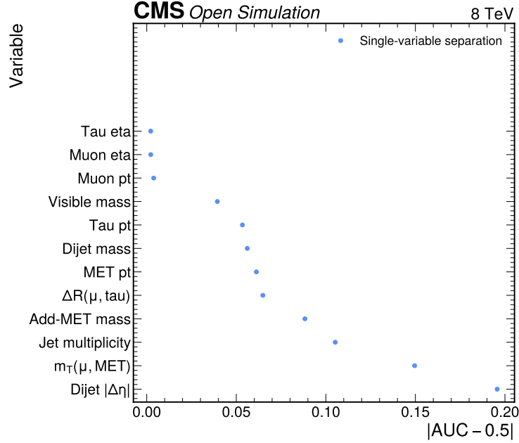
Figure 30: Phase 2 variable separation ranking. The ranking summarized single-variable raw MC separation in the exploratory slice. It explains why VBF-related quantities, transverse mass, jet multiplicity, add-MET mass, and visible mass remained under consideration before Phase 3 validation.
