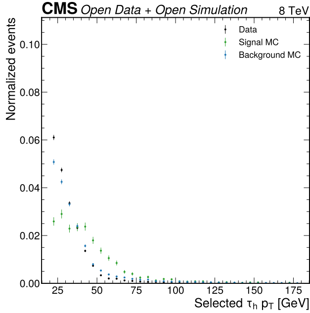
Figure 7: Selected tauh transverse momentum. The Phase 3 plot verifies that the tight tau isolation and tight anti-muon veto leave a physically populated tauh spectrum. This object definition is inherited without modification by the Phase 4a expected model.
