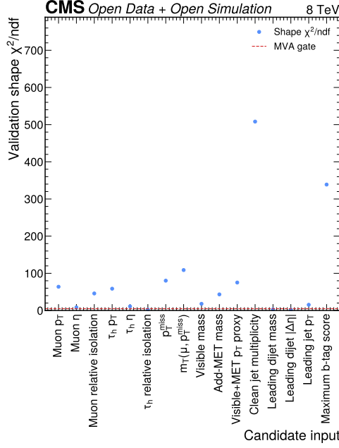
Figure 18: MVA input modelling gate. The Phase 3 gate compares validation/control-region data and background-MC shapes for candidate classifier inputs. Most candidate inputs exceed the predeclared \chi^2/ndf threshold of 5, so the classifier is not trained or promoted in this Phase 4a model.
