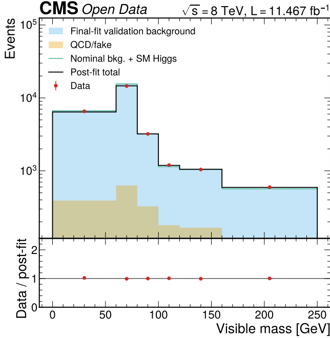
FIG. 2. Combined post-fit Data/MC validation. The left panel shows the visible-mass baseline summed over VBF, boosted, and zero-jet categories; the right panel shows the corresponding combined D_{NN} score distribution. Both lower panels use Data/post-fit model ratios.
