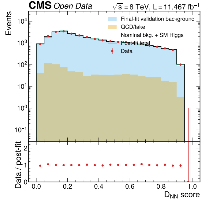
FIG. 2. Combined post-fit Data/MC validation. The left panel shows the visible-mass baseline summed over VBF, boosted, and zero-jet categories; the right panel shows the corresponding combined D_{NN} score distribution. Both lower panels use Data/post-fit model ratios.
