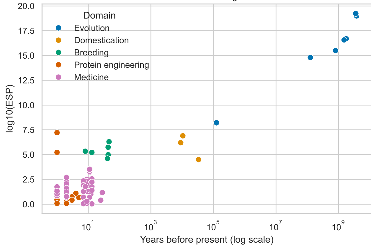
Unified ESP learning curve
