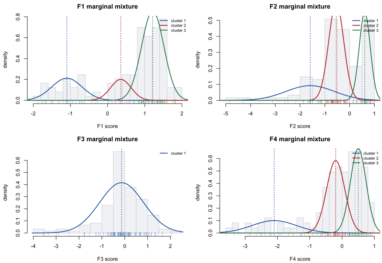
Figure 2: Marginal mixture fits
