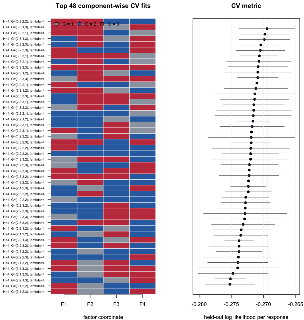
Figure 1: Component-wise CV metrics for H=4 , \lambda=4
