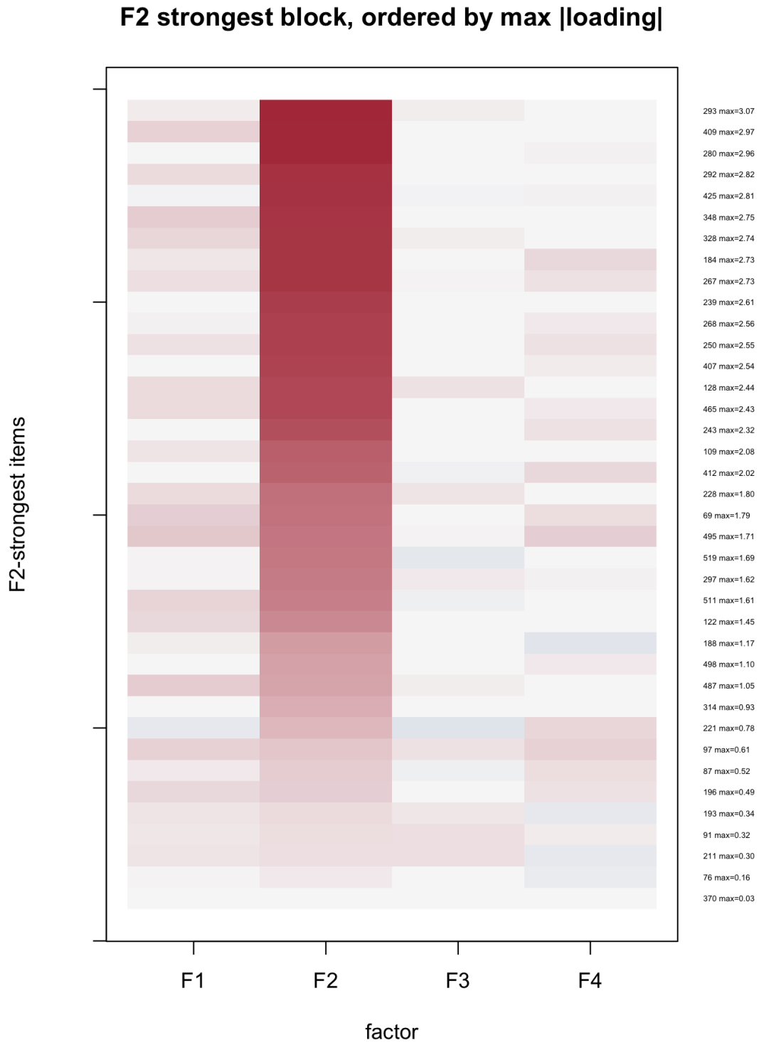
Figure 6: Zoomed F2 strongest block
