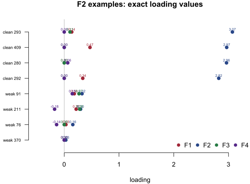
Figure 7: Exact F2 loading values
