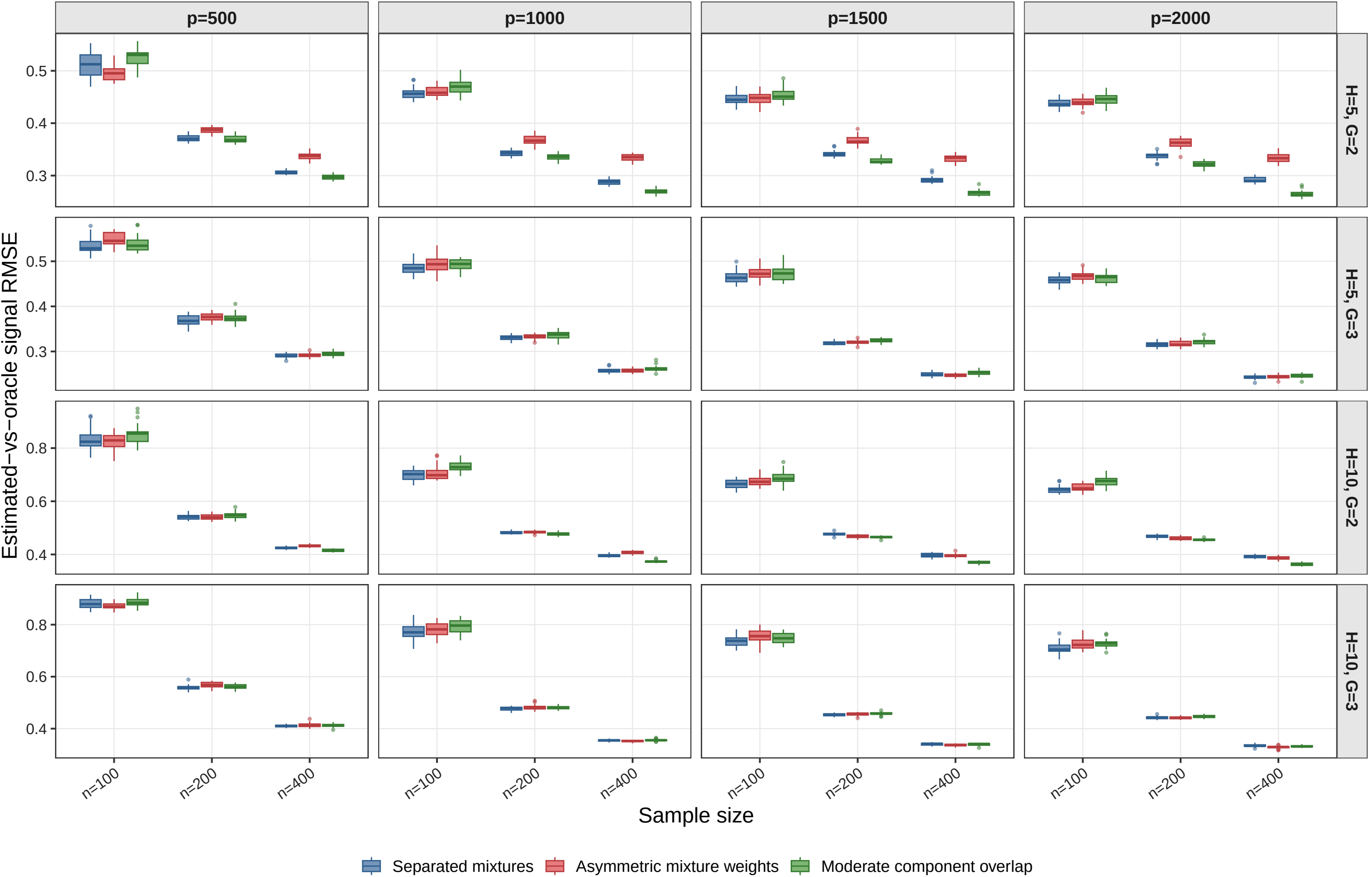
Estimated Probit Signal Recovery Across Mixture Settings
