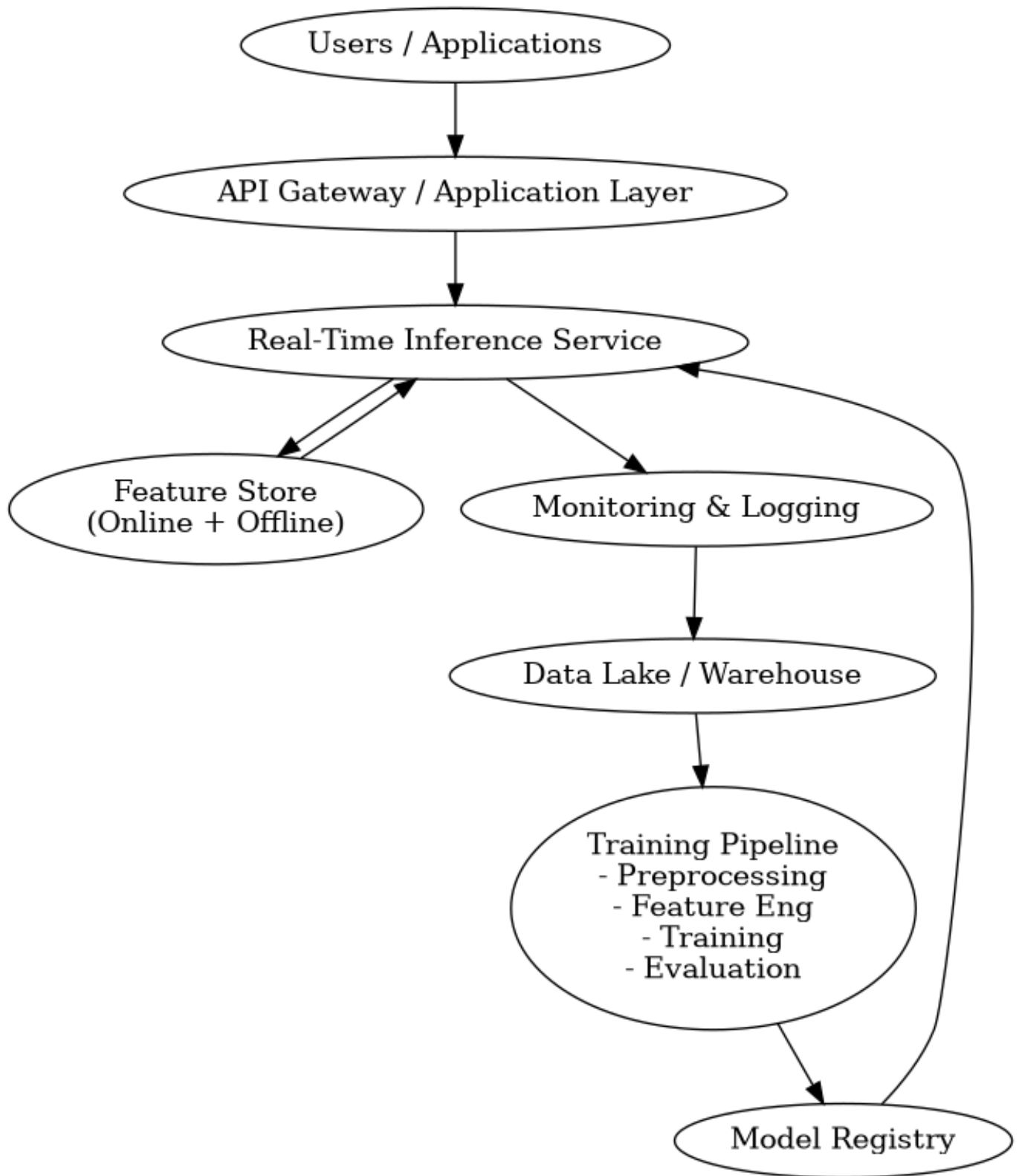
Fig. 2. AI Architecture 2 — an alternative view of the deep learning pipeline.
