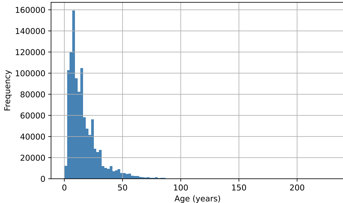
Distribution of Age (parquet: sale year - vintage year)
