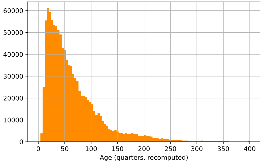
Distribution of Age (recomputed quarters, trimmed at 400q)
