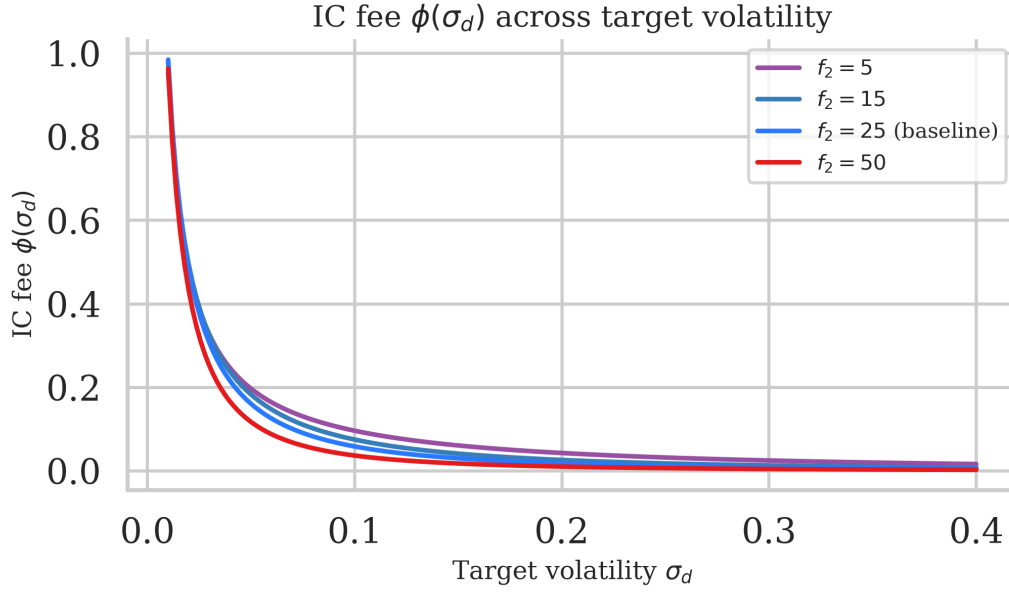
Figure 2: Incentive-compatible fee \phi(\sigma_d) as a function of the target volatility \sigma_d under different flow convexities f_2 . Higher convexity reduces the fee required to discipline risk taking.
