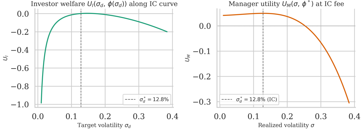
Figure 9: Incentive alignment diagnostics under the IC contract. Left panel: investor utility U_I(\sigma_d, \phi(\sigma_d)) along the IC-feasible frontier as a function of the volatility target \sigma_d , with the optimal target \sigma_d^* marked. Right panel: manager utility U_M(\sigma, \phi^*) as a function of realized volatility \sigma at fixed IC fee \phi^* = \phi(\sigma_d^*) , confirming that the manager's privately optimal choice equals \sigma_d^* .
