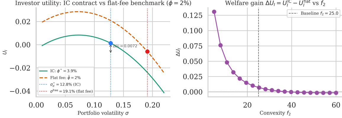
Figure 8: Welfare comparison: IC contract vs. flat-fee benchmark. The benchmark is a market flat fee \phi_{\text{mkt}} = 2\% ; at that fee, the manager freely chooses \sigma^{\text{free}} = \arg \max_{\sigma} U_M(\sigma; \phi_{\text{mkt}}) > \sigma_d^* . Left panel: investor utility U_I(\sigma, \phi) as a function of \sigma under the IC fee \phi^* (solid) and the flat fee \phi_{\text{mkt}} (dashed); vertical lines mark the IC target \sigma_d^* and the laissez-faire choice \sigma^{\text{free}} ; the shaded gap quantifies the welfare gain \Delta U_I = U_I(\sigma_d^*, \phi^*) - U_I(\sigma^{\text{free}}, \phi_{\text{mkt}}) . Right panel: welfare gain \Delta U_I as a function of the convexity parameter f_2 , showing that the welfare gain is decreasing in f_2 : IC enforcement delivers the largest improvement at moderate convexity, and the gain diminishes as convexity increases because the IC fee must fall sharply to maintain incentive alignment.
