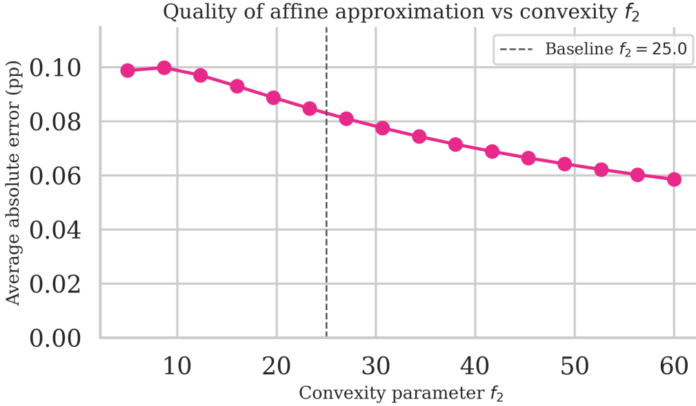
Figure 11: Quality of the affine approximation: average absolute error (in percentage points) between the exact IC fee \phi(\sigma_d) and its linear approximation. For each convexity parameter f_2 , the approximation is centered at the optimal target \sigma_d^* and evaluated within \pm 5\% of that target.
