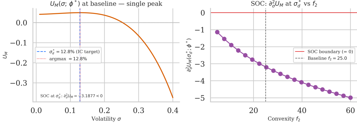
Figure 10: Global IC verification. Left panel: manager utility U_M(\sigma; \phi^*) over the full range \sigma \in [0.01, 0.40] at the baseline IC fee \phi^* , confirming a unique maximum at \sigma_d^* (dashed line); the argmax coincides with the IC target to three decimal places. The second-order condition \partial_\sigma^2 U_M(\sigma_d^*; \phi^*) < 0 (reported in panel label) holds strictly. Right panel: SOC value \partial_\sigma^2 U_M evaluated at (\sigma_d^*, \phi^*) across the f_2 sweep; all values are negative, confirming the SOC holds throughout the calibrated parameter grid.
