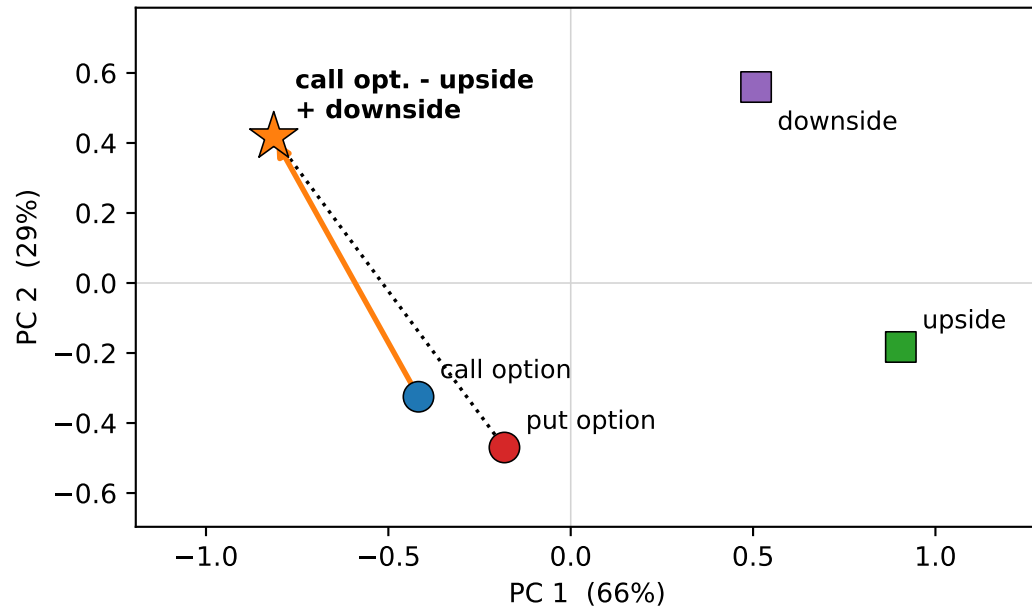
(b) Finance analogy fails: nearest words are generic call - upside + downside does not give put in GloVe
