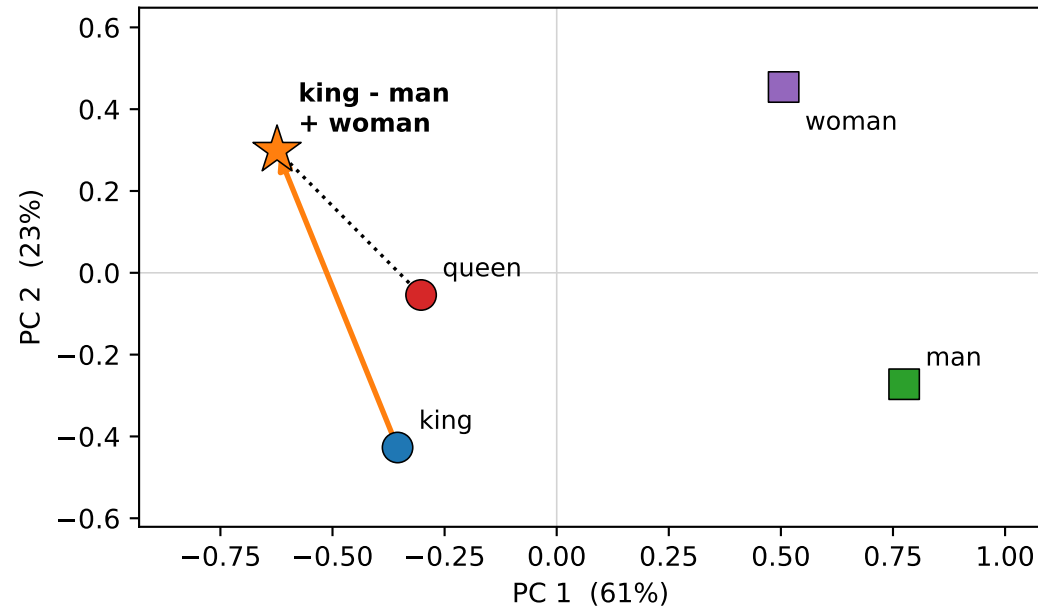
(a) Classic analogy holds: nearest word is queen king - man + woman \approx queen ( \cos = 0.67 )
