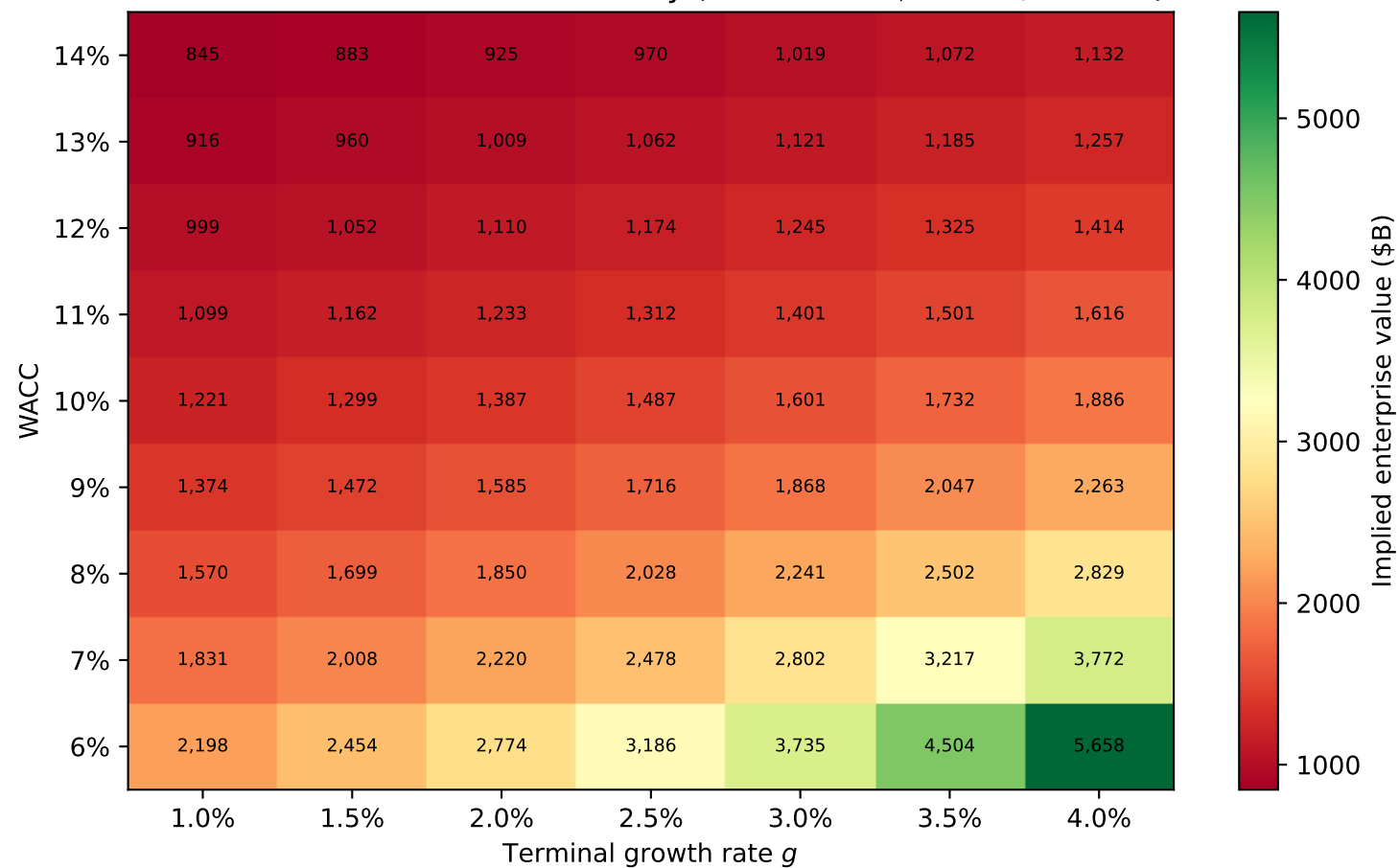
AAPL DCF terminal-value sensitivity (base FCF = $108.8B, FY2024)
