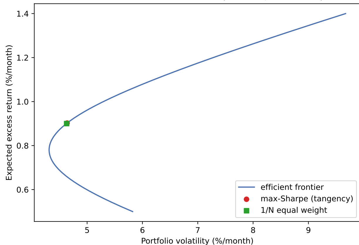
Mean-variance efficient frontier (4 assets, illustrative)
