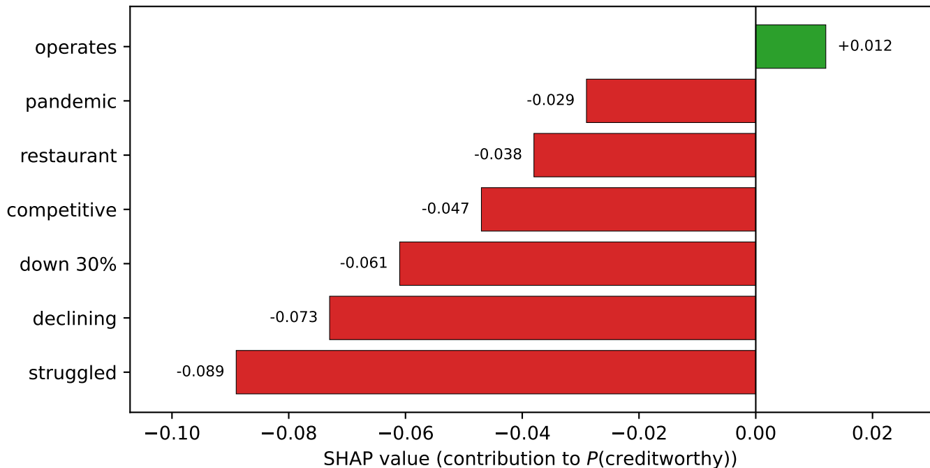
Token attributions for a credit-decision classifier (baseline 0.50 \rightarrow model output 0.14)
