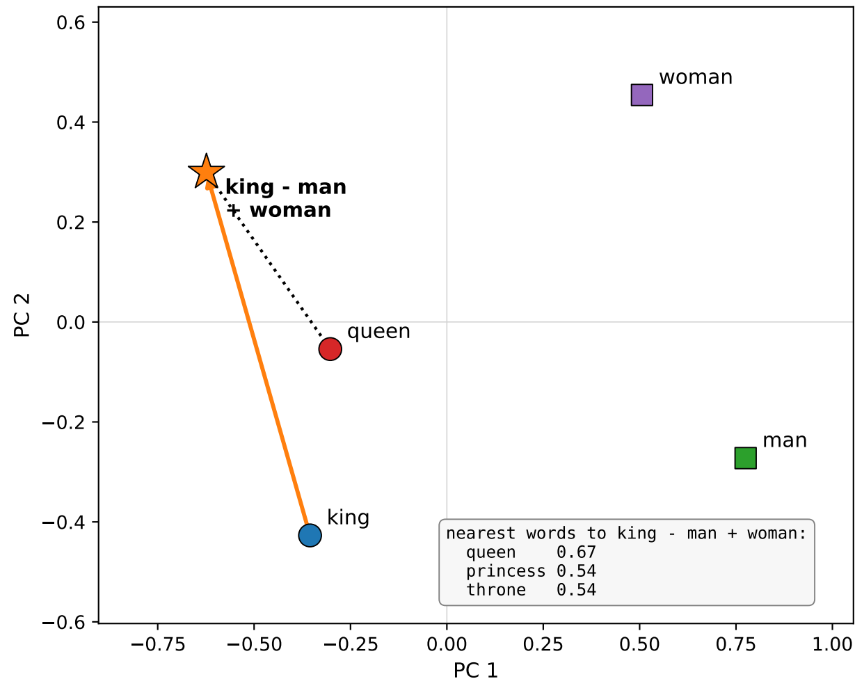
Word analogy in GloVe (300d): king - man + woman \approx queen
