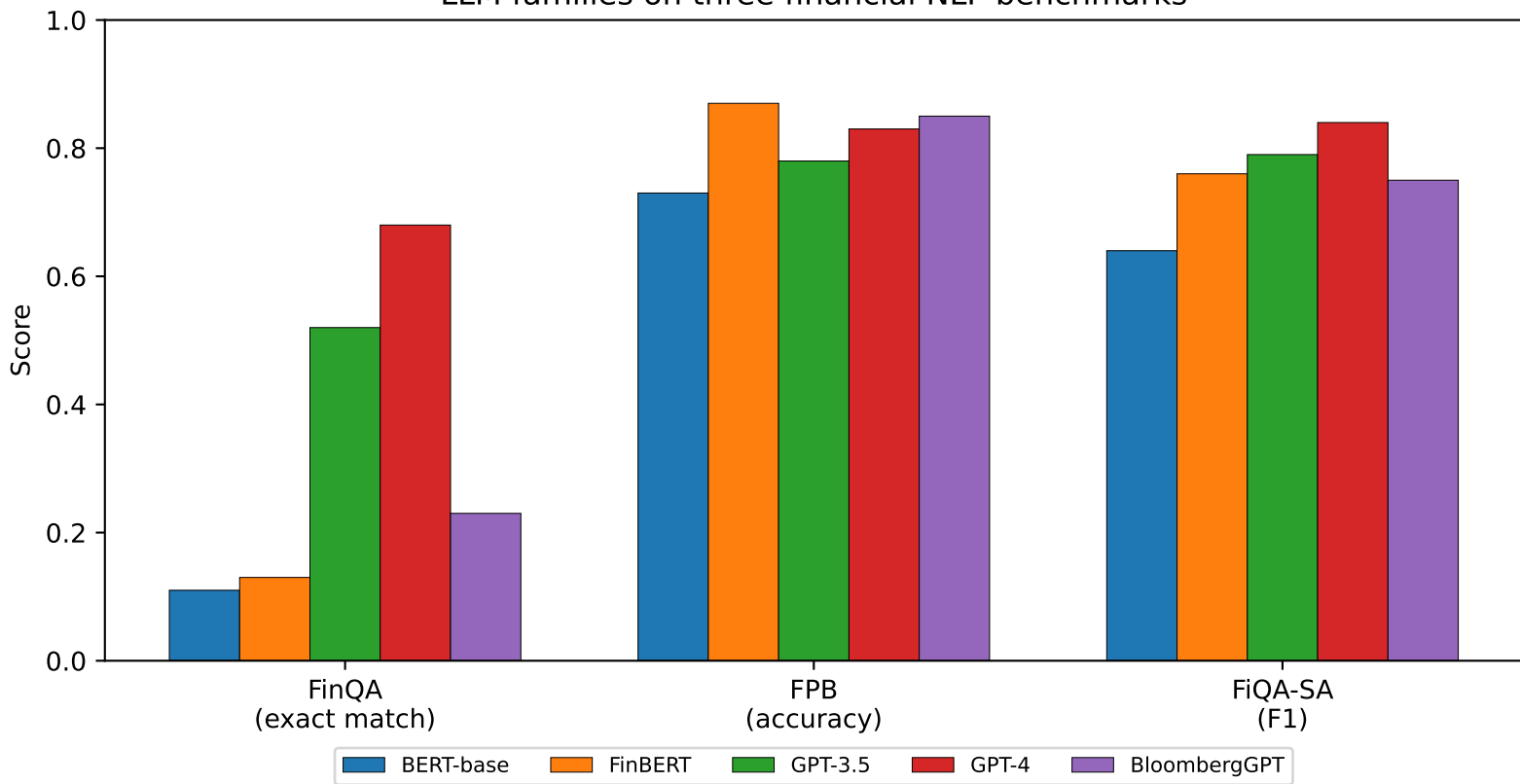
LLM families on three financial NLP benchmarks
