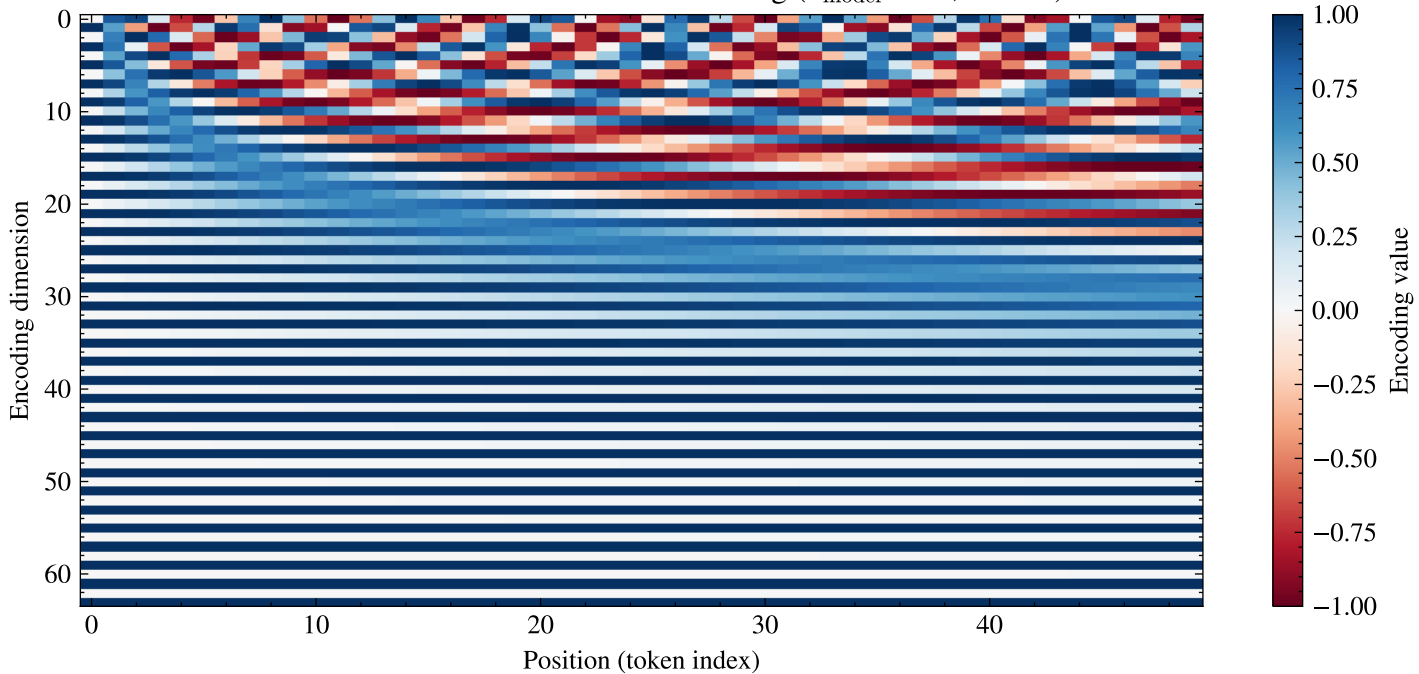
Transformer Sinusoidal Positional Encoding ( d_{\text{model}} = 64, n = 50 )
