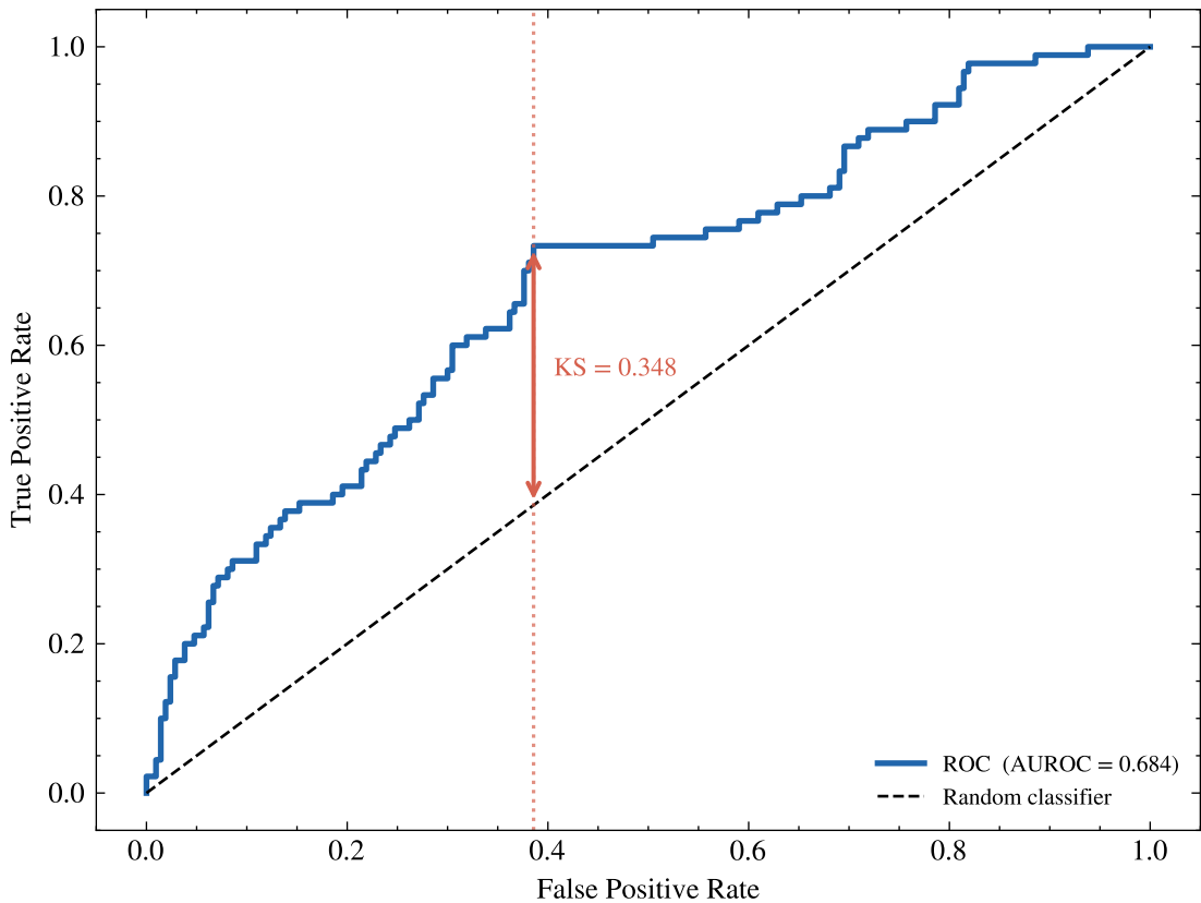
ROC Curve — German Credit Dataset (Logistic Regression on 6 numeric features)
