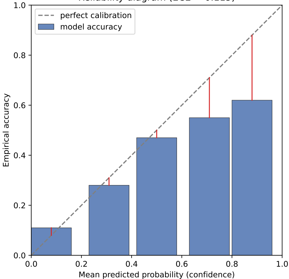
Reliability diagram (ECE = 0.115)
