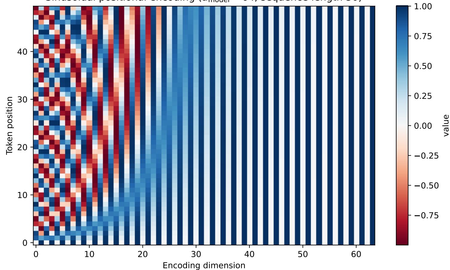
Sinusoidal positional encoding ( d_{\text{model}} = 64 , sequence length 50)
