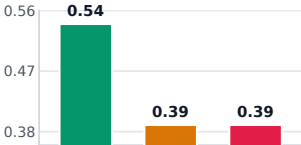
Cost ↓
