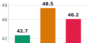
Reward ↑
