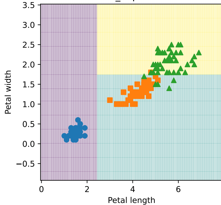
max_depth = 2
