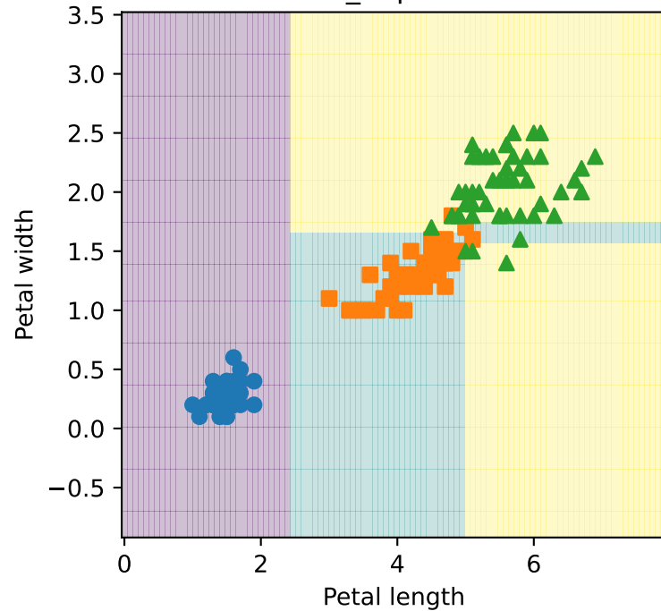
max_depth = 4
