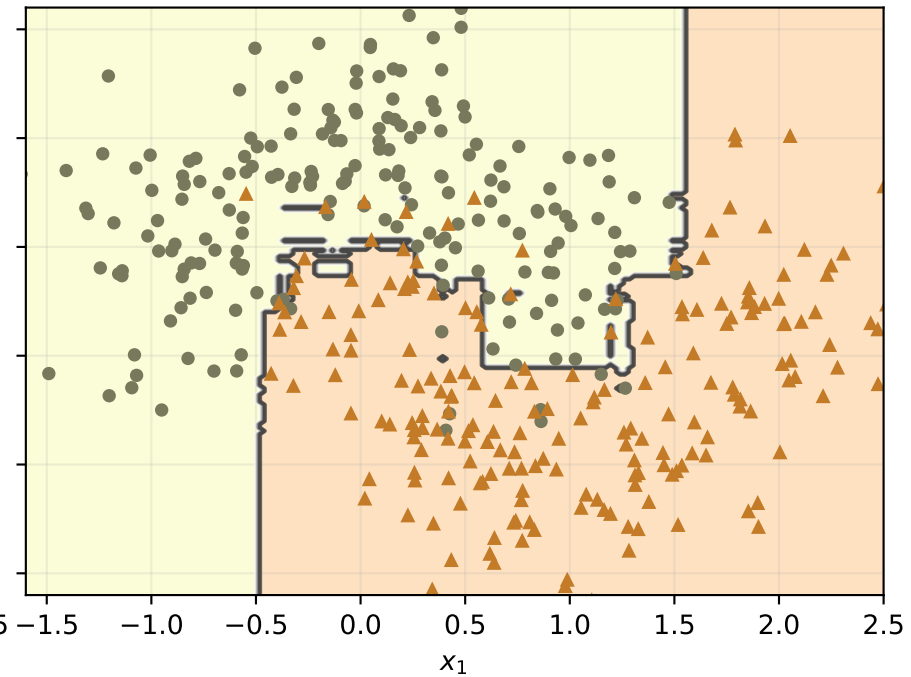
Bagged decision trees
