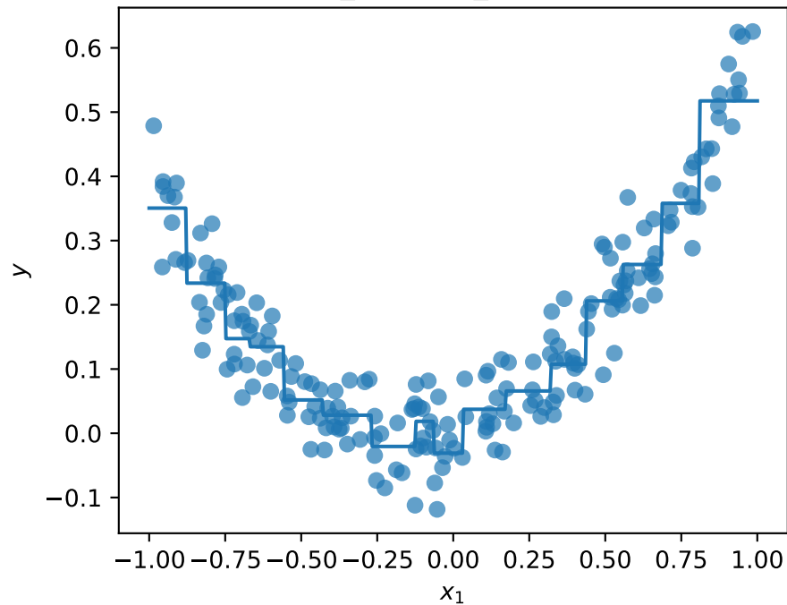
min_samples_leaf = 10
