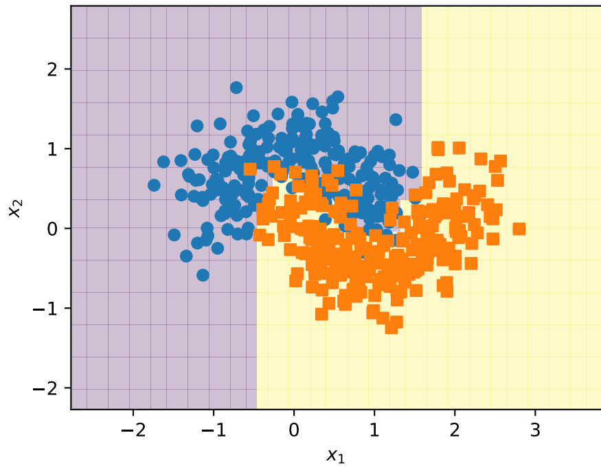
Bootstrap sample B
