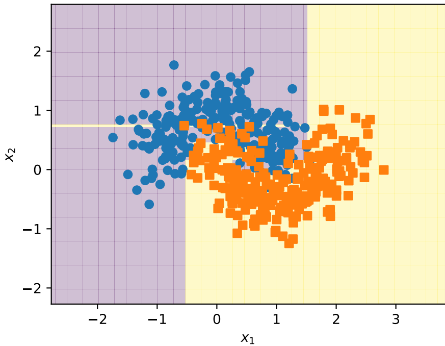
Bootstrap sample A
