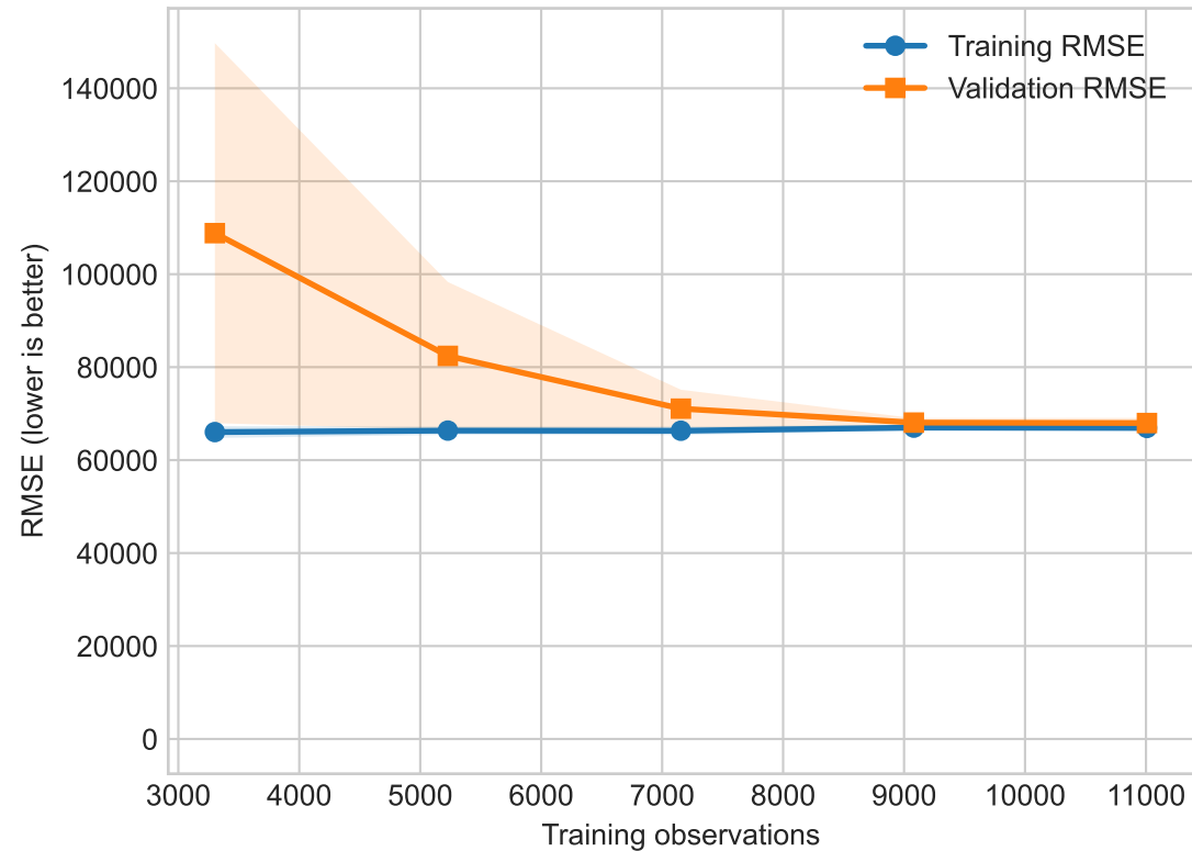
Underfitting signal: linear regression
