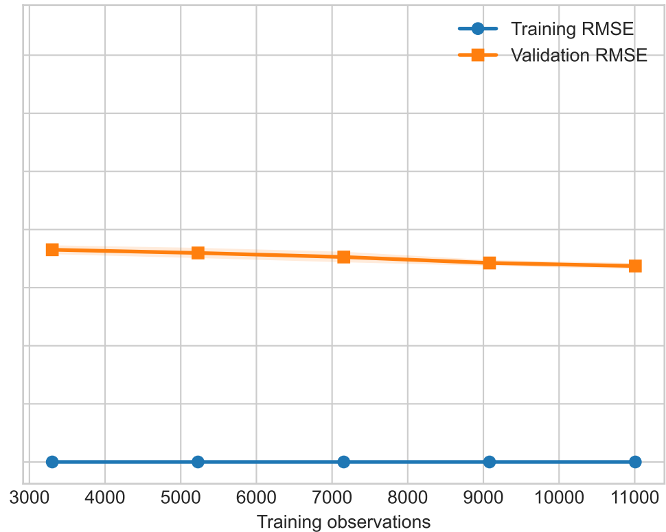
Overfitting signal: decision tree
