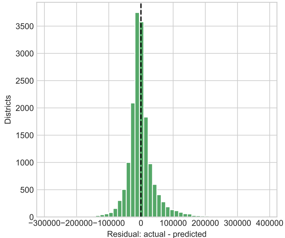
Residual distribution
