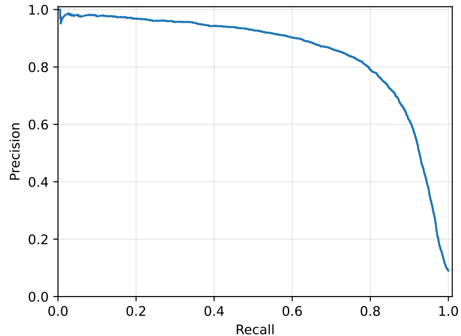
Precision-Recall curve
