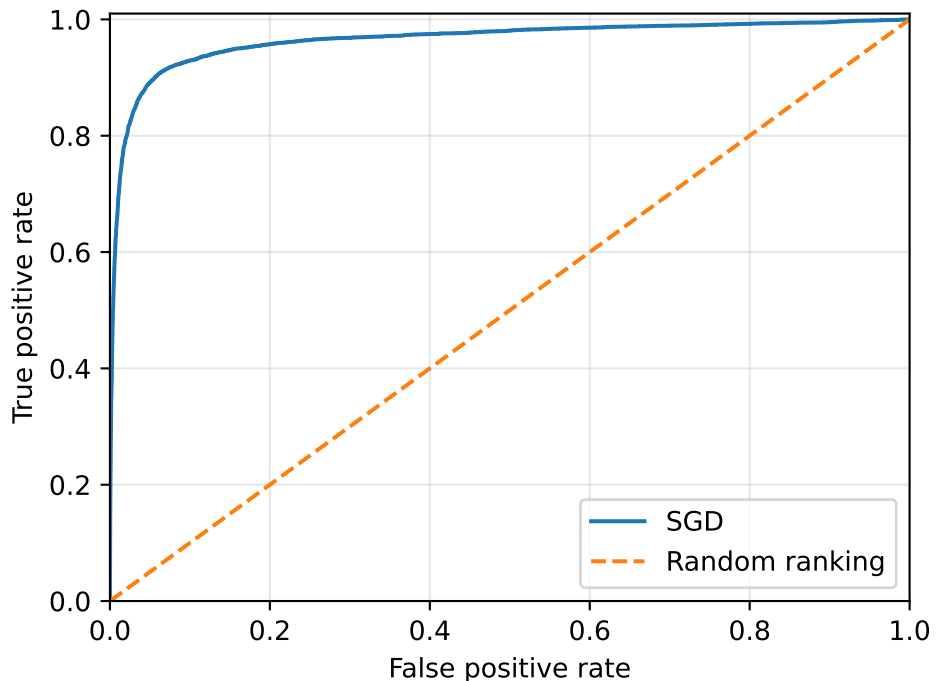
ROC curve
