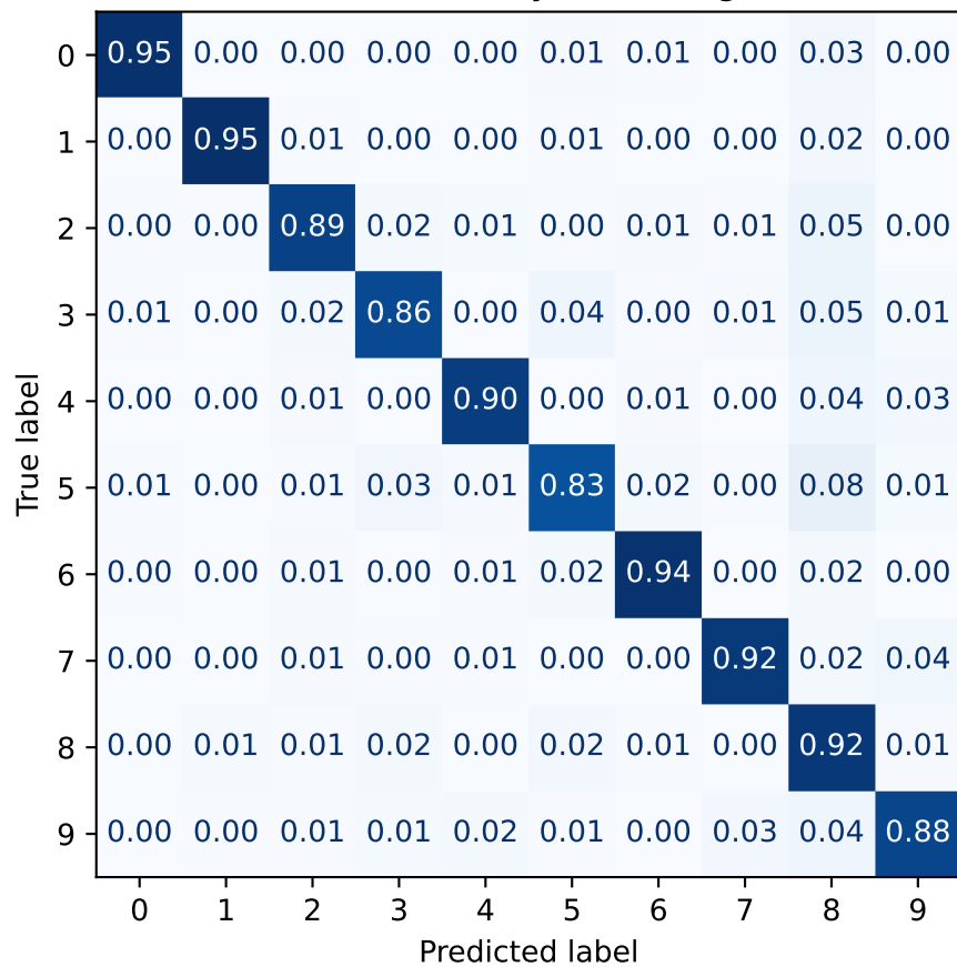
Normalized by actual digit
