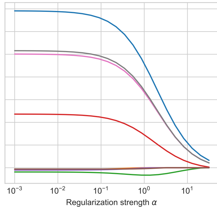
Elastic Net
