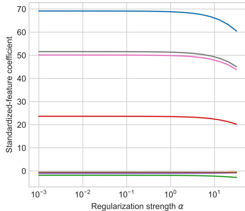
Ridge
