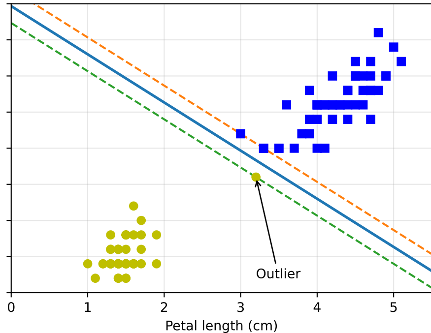
Decision boundary dominated by one outlier
