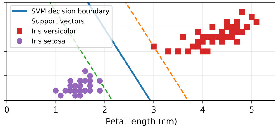
Near hard-margin solution
