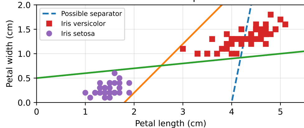
Possible linear separators
